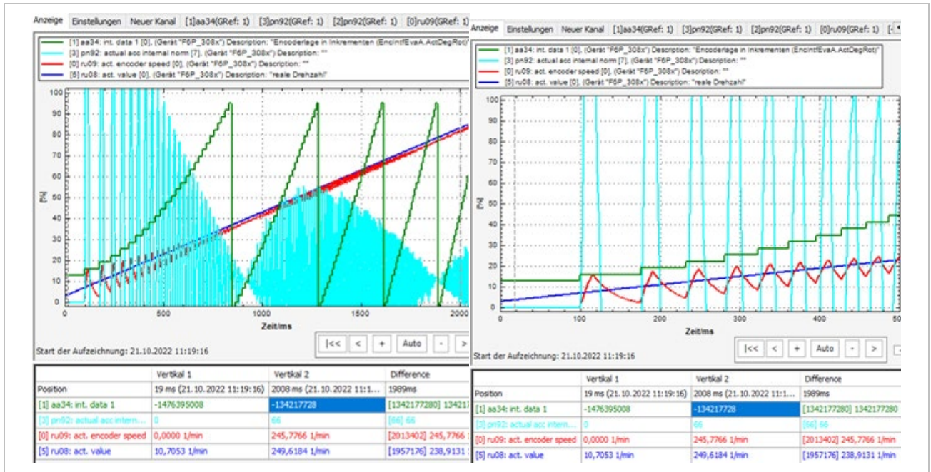
Figure 22: Speed ripple at small number of increments per revolution
