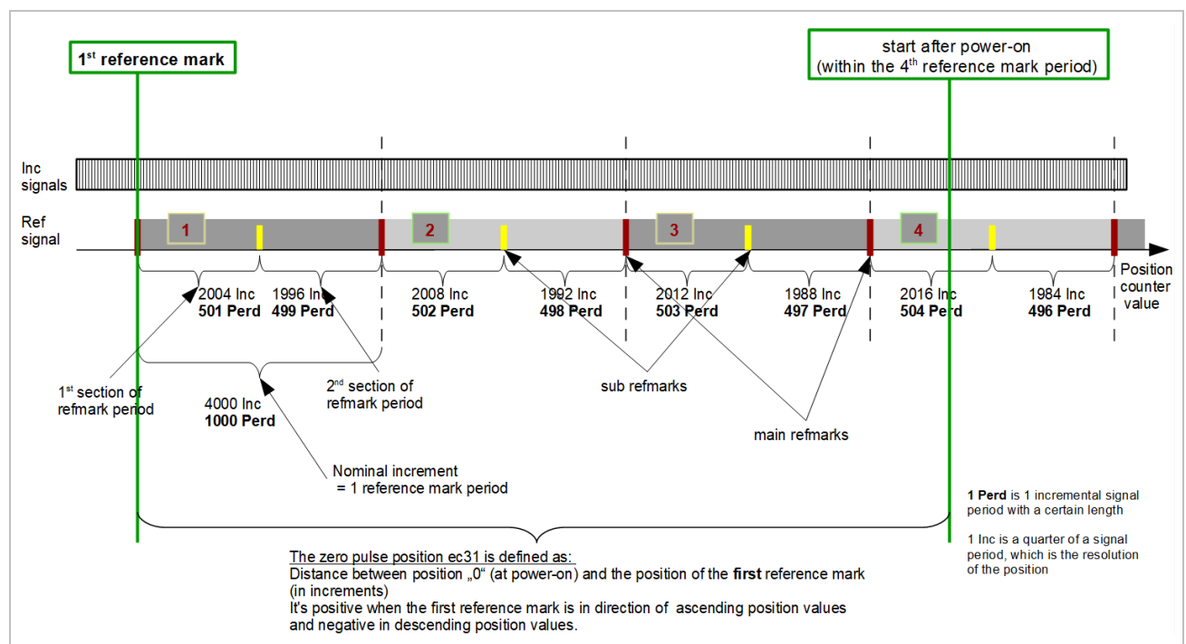
Figure 73: distance-coded reference marks in detail
