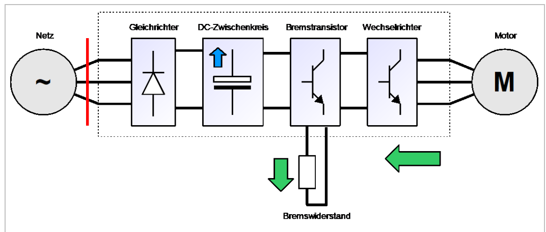
Figure 28: Regenerative operation in case of mains power failure
