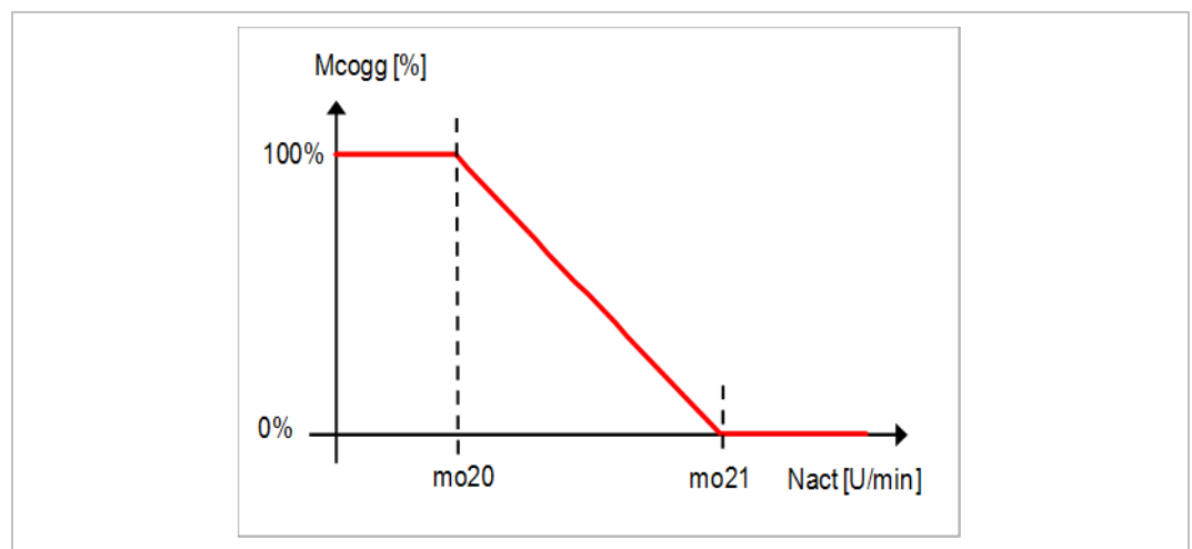
Figure 94: Cogging torque compensation
