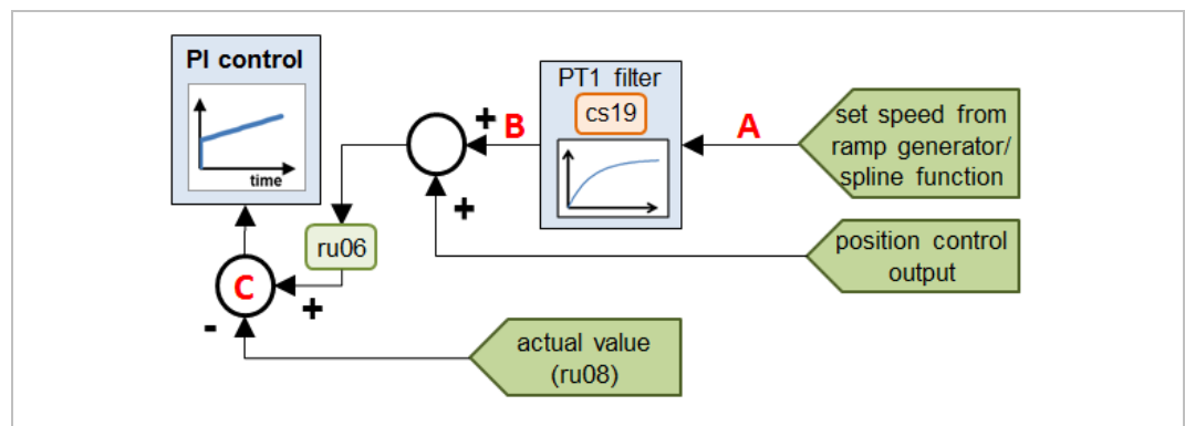
Figure 69: Auxiliary representation for the calculation of ru33[]
