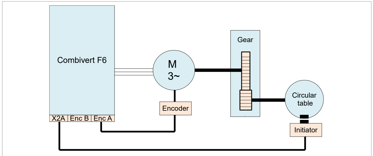
Figure 39: Motor encoder with initiator at rotary table
