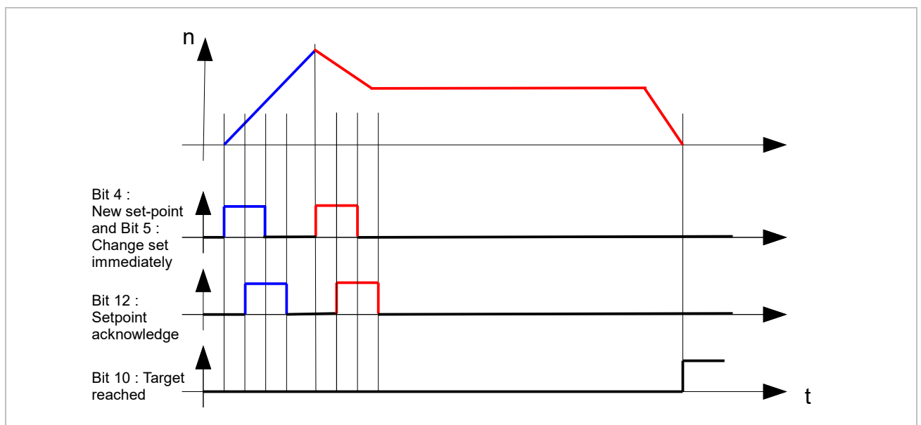
Figure 37: Restart of a positioning
