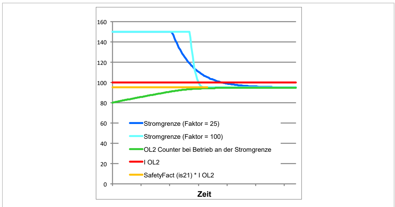
Figure 12: Characteristic of the current limit in relation to the time
