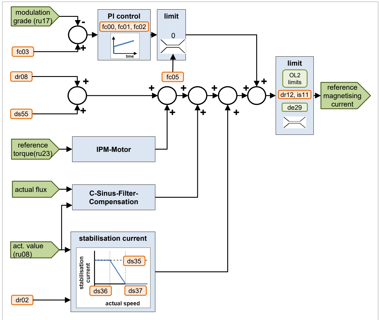
Figure 81: Formation of the d-component
