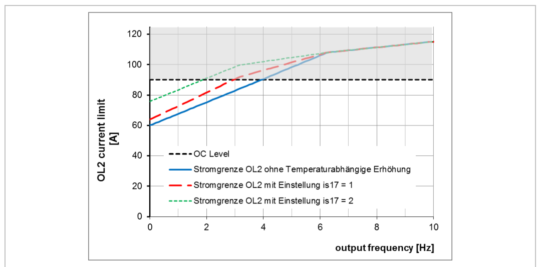
Figure 11: Increase OL2 for 60A rated current and 40°C
