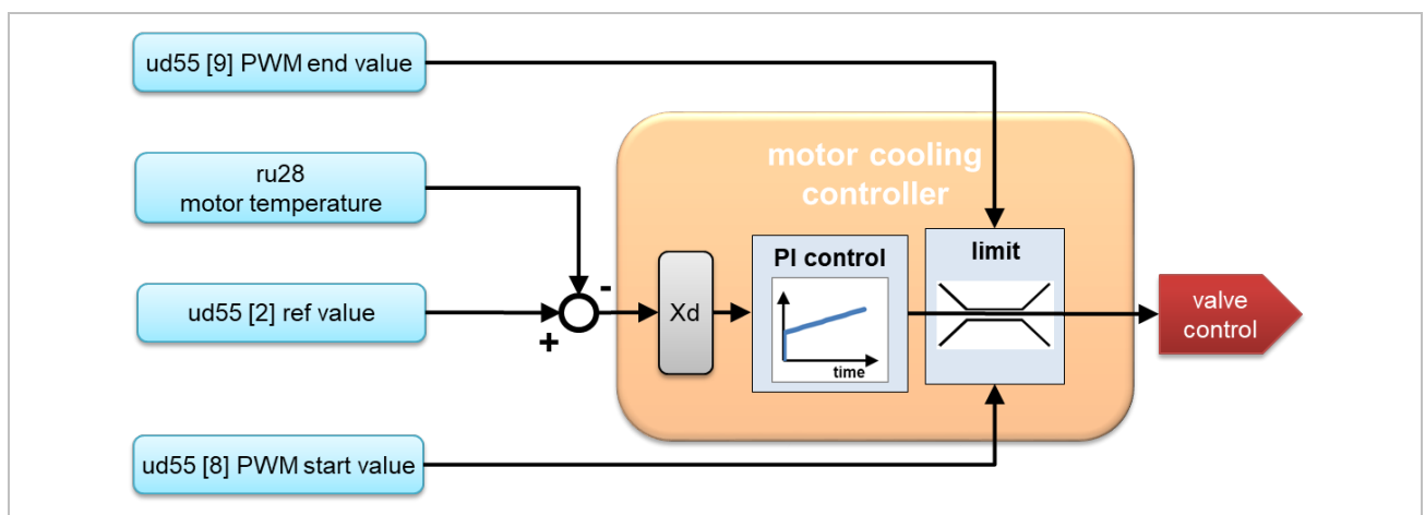
Figure 155: Overview controller motor cooling
