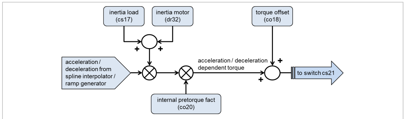
Figure 117: Torque precontrol mode 2
