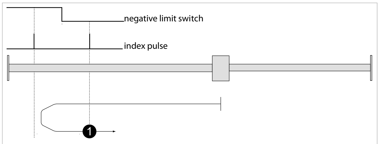
Figure 51: Homing – Method 1
