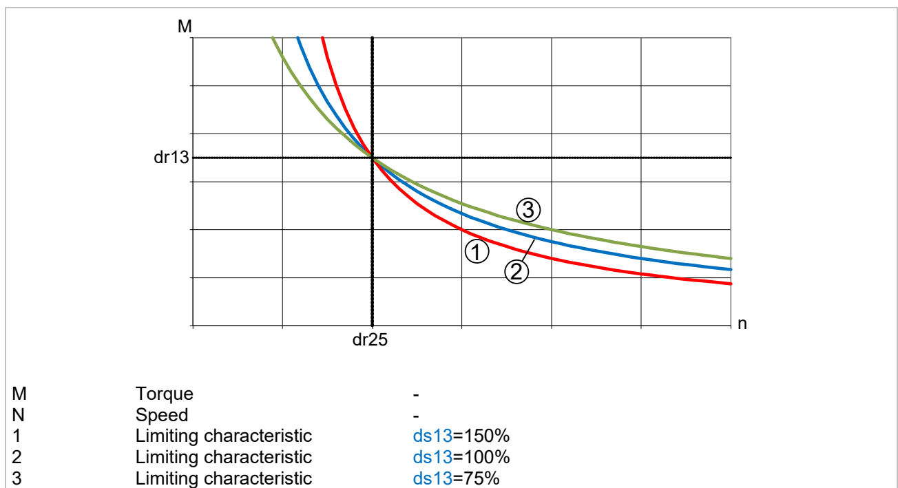
Figure 89: Adjustment of the torque limiting characteristic
