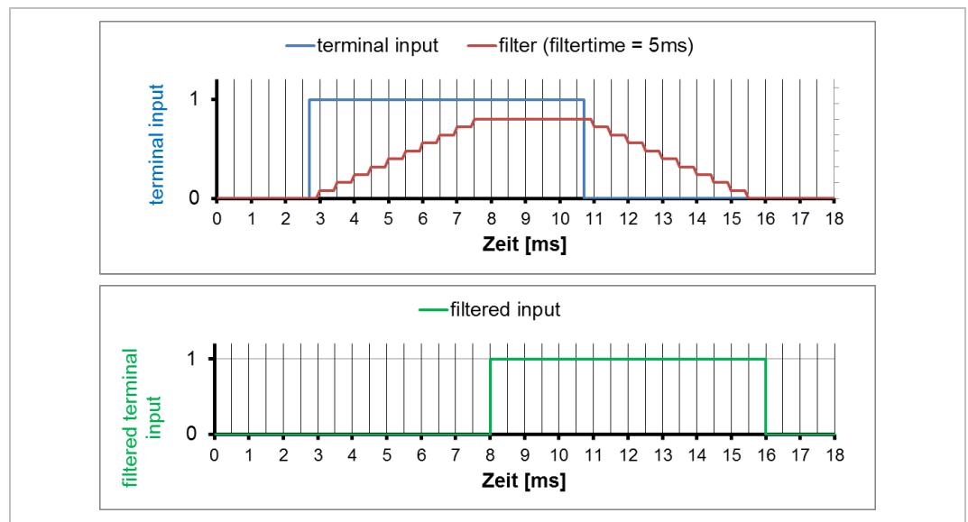
Figure 128: Filter of the digital inputs
