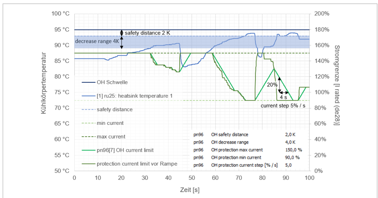
Figure 14: Graph of the current limit depending on the heat sink temperature
