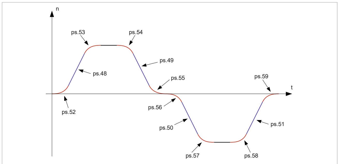
Figure 38: Ramps in profile position mode
