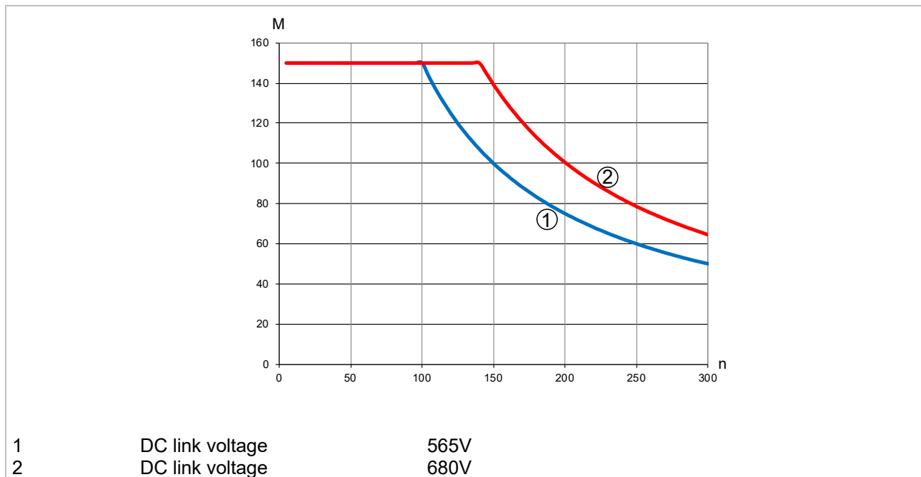
Figure 88: Maximum torque depending on the DC link voltage for the synchronous motor
