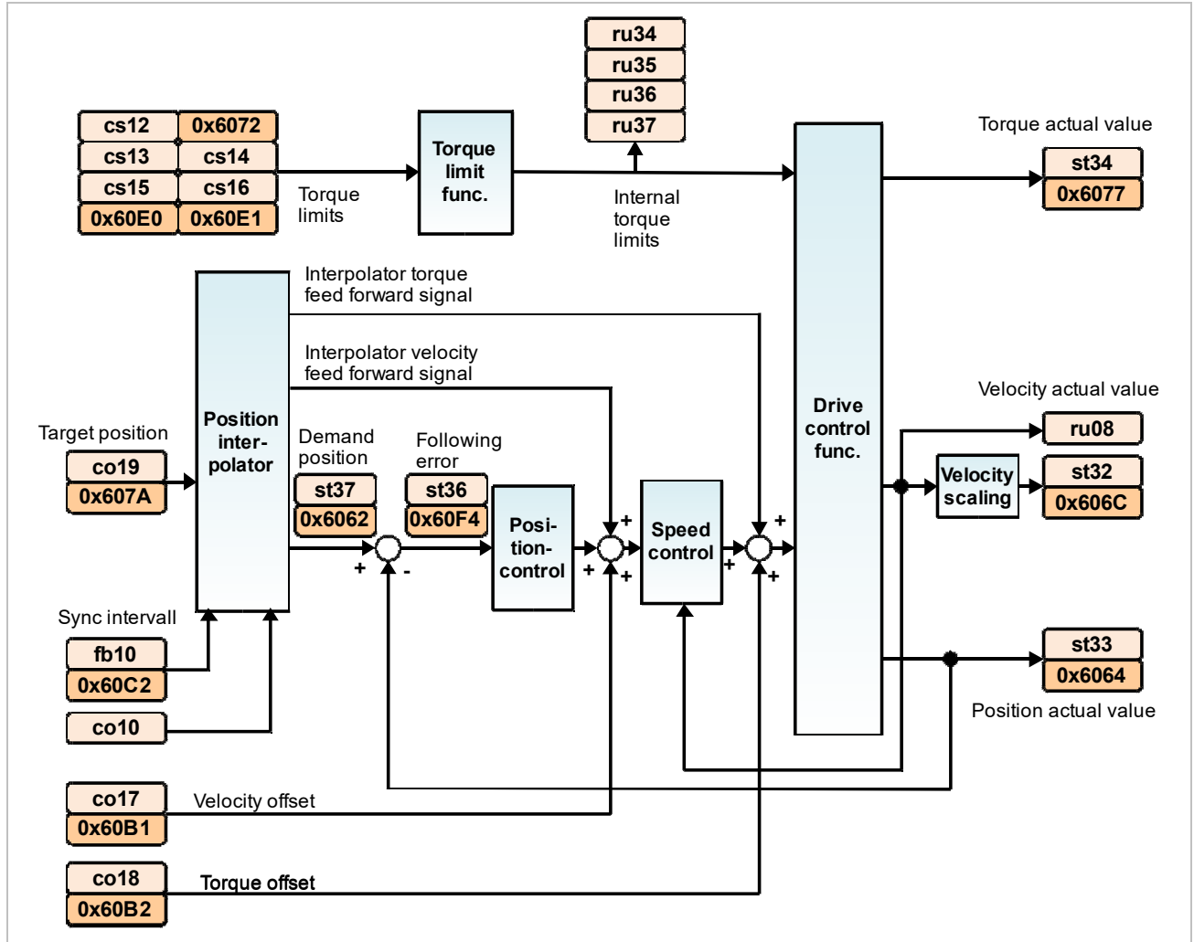
Figure 58: Cyclic synchronous position mode
