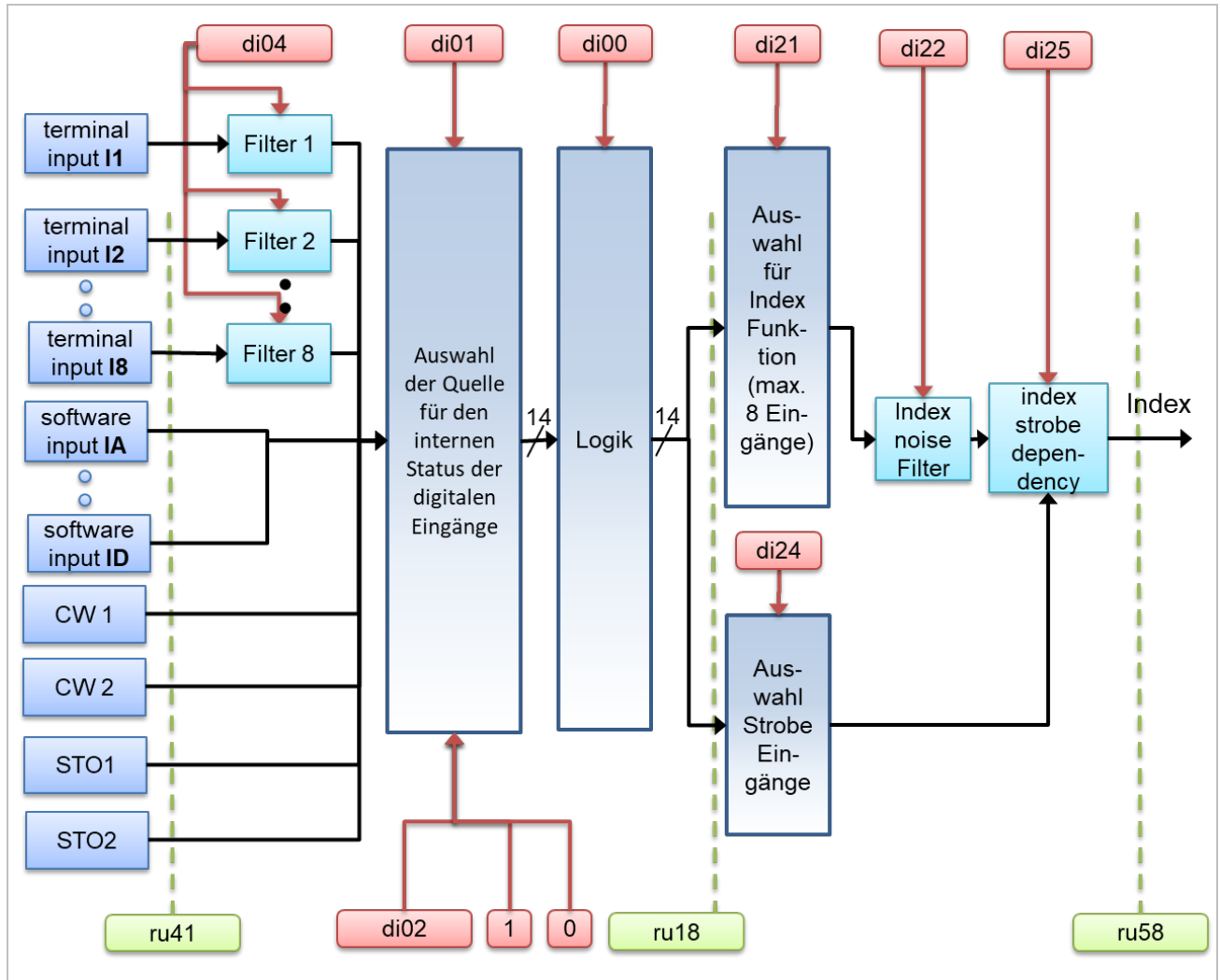
Figure 137: Overview index generation with filters and strobe
