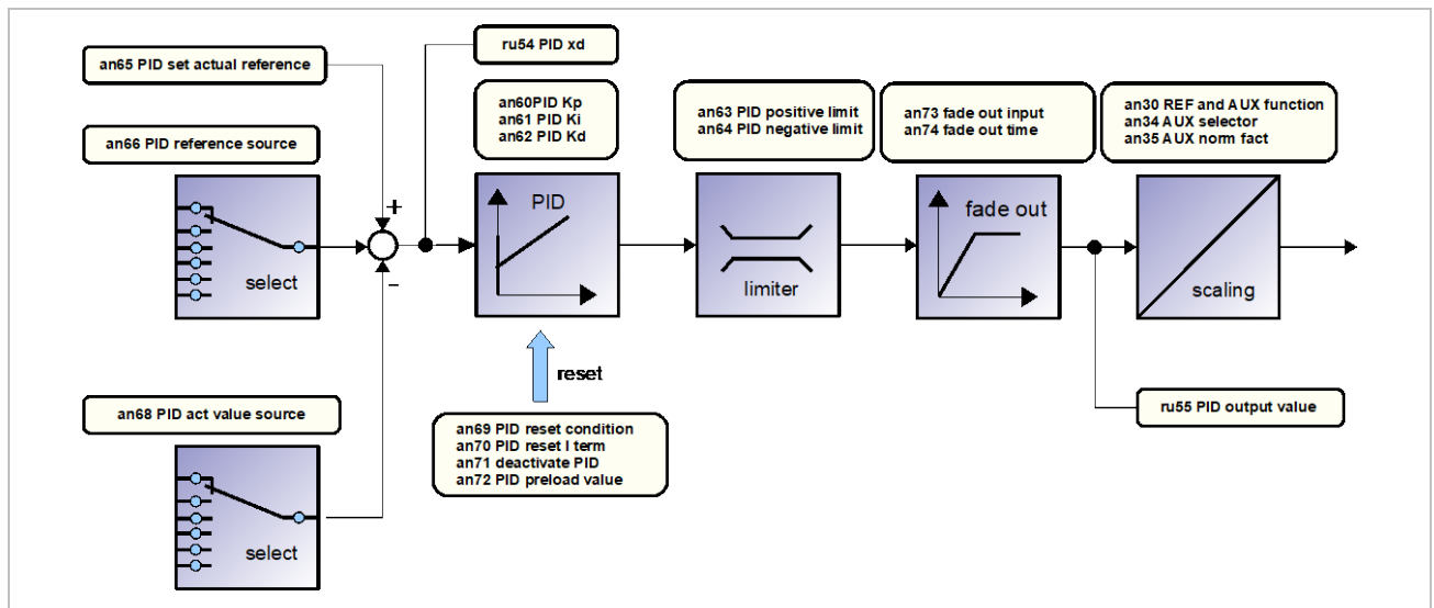
Figure 142: PID controller
