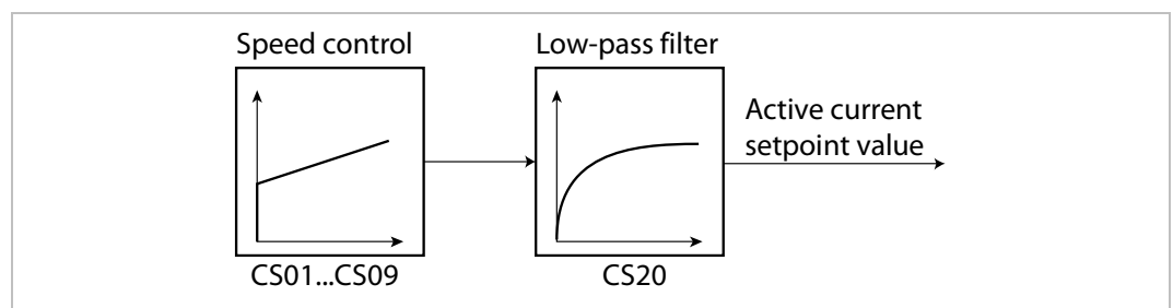
Figure 115: PT1 output filter
