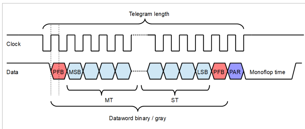
Figure 75: Structure data word SSI
