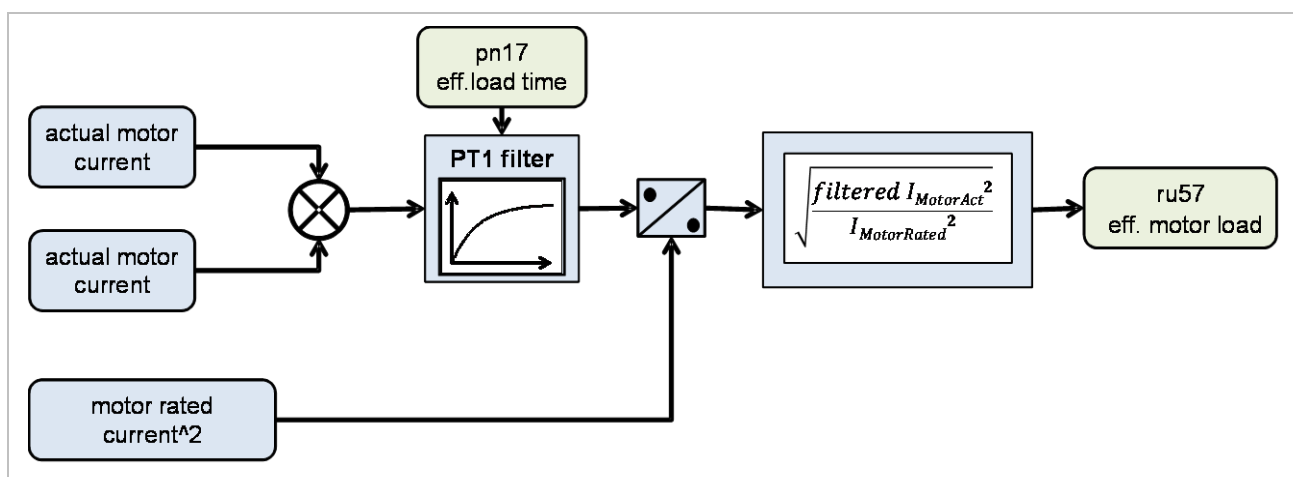
Figure 21: Effective motor load
