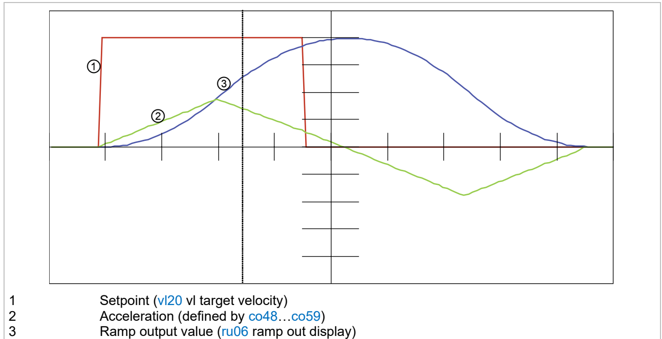
Figure 46: s-curve type = 0: continuous s-curve
