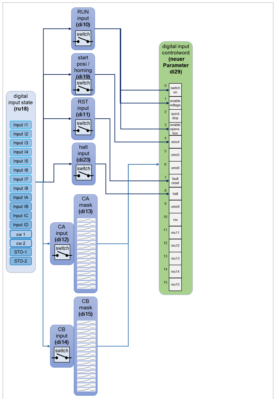
Figure 133: digital input controlword
