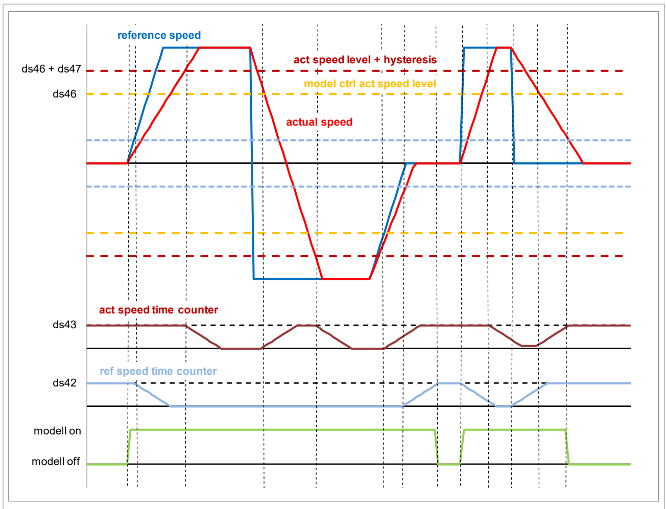
Figure 100: Model deactivation depending on the motor type
