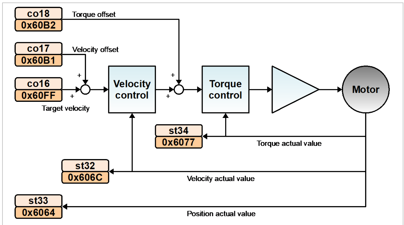
Figure 61: Cyclic synchronous velocity mode - principle
