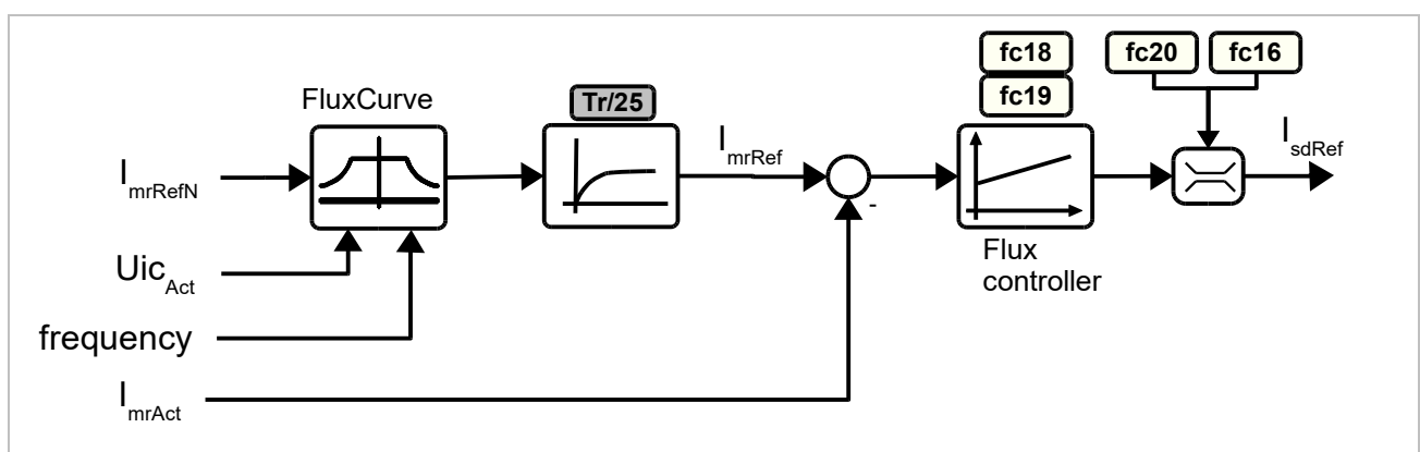
Figure 92: Flux controller (ASM)
