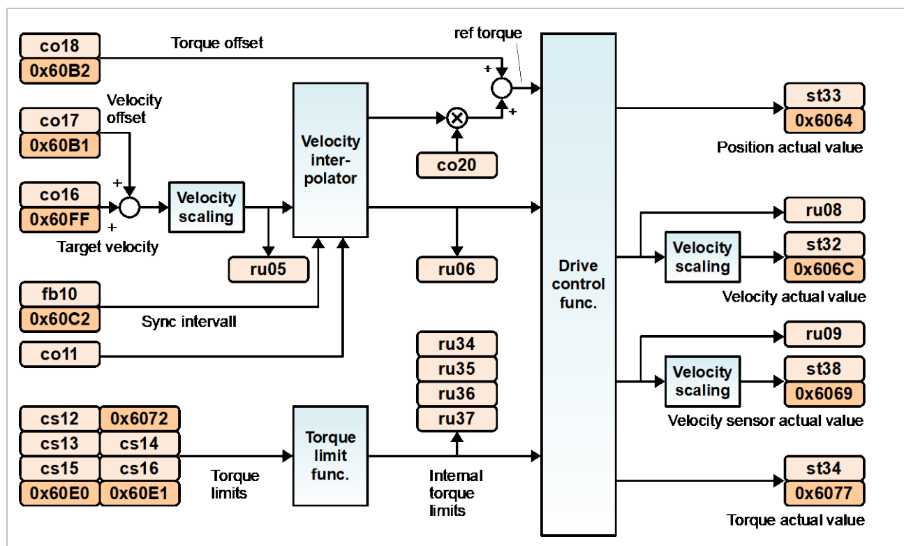
Figure 62: Cyclic synchronous velocity mode
