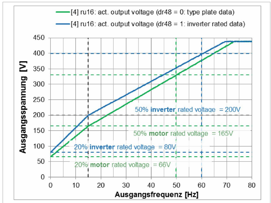
Figure 99: v/f - Influence of dr48 v/f characteristic mode
