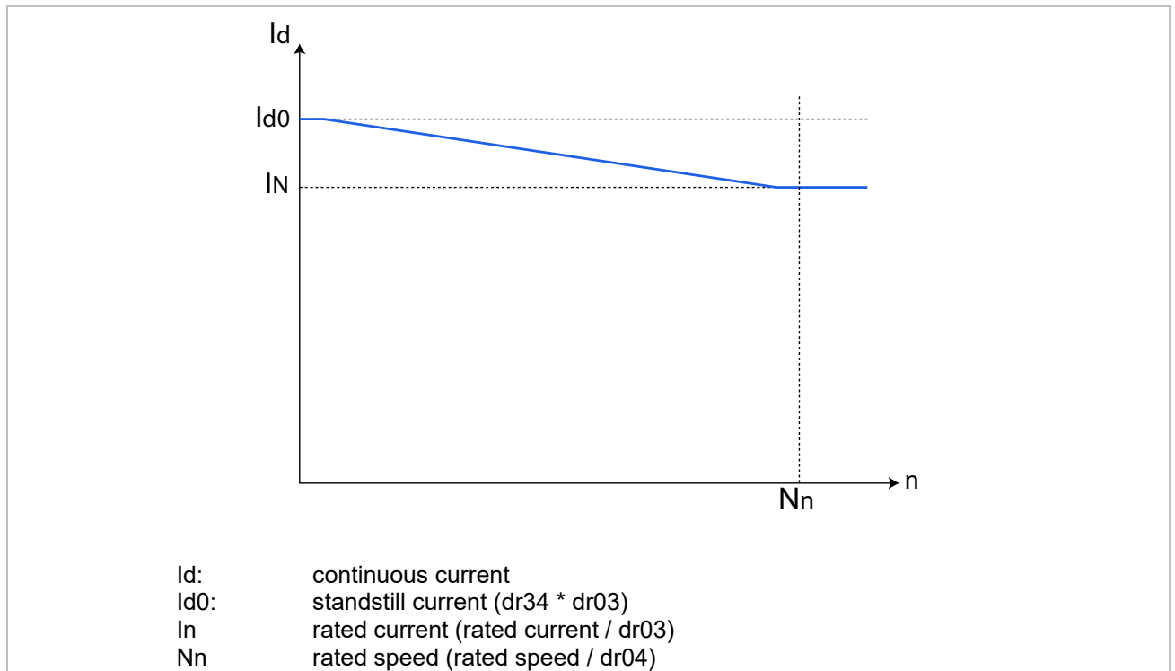
Figure 18: Dependence of the motor protection function
