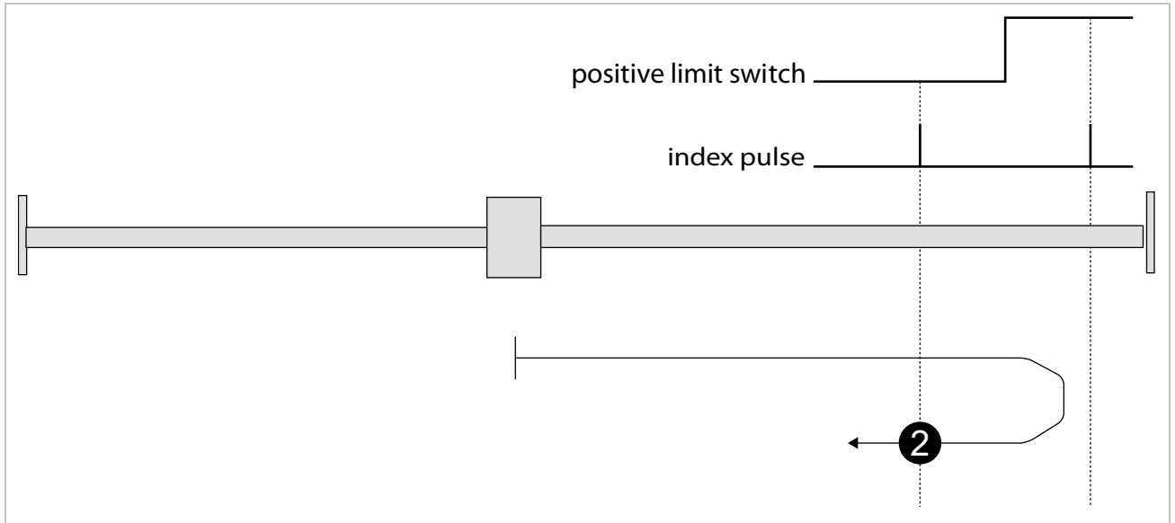
Figure 52: Homing – Method 2
