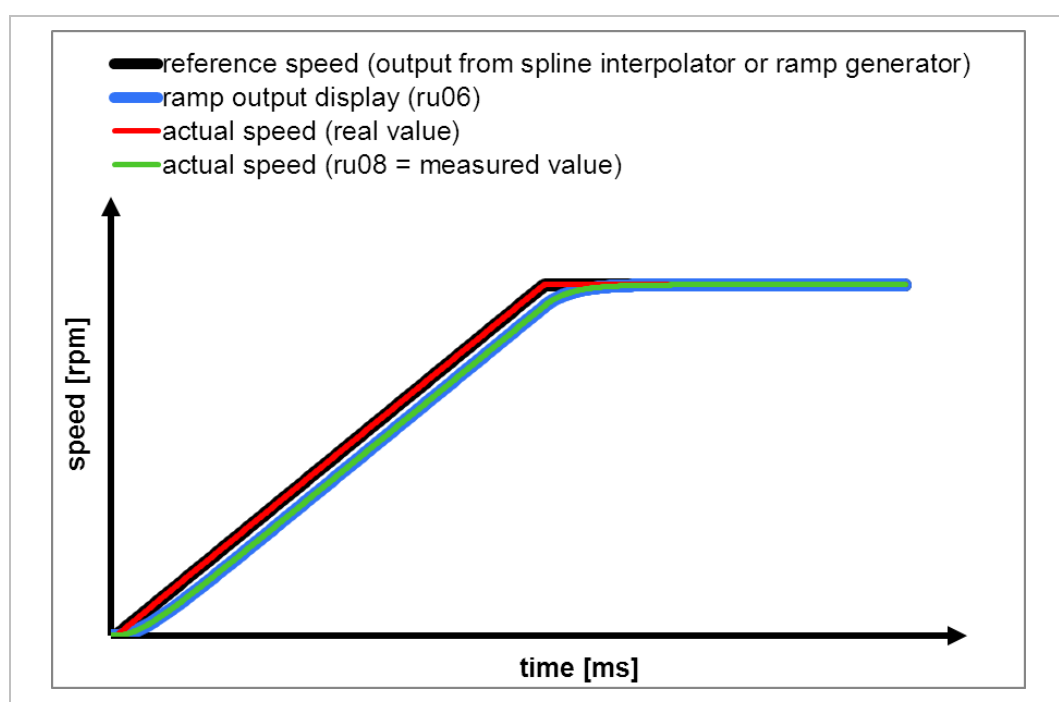
Figure 122: Optimal precontrol behaviour
