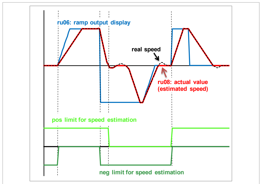
Figure 103: Torque limit depending on the setpoint value
