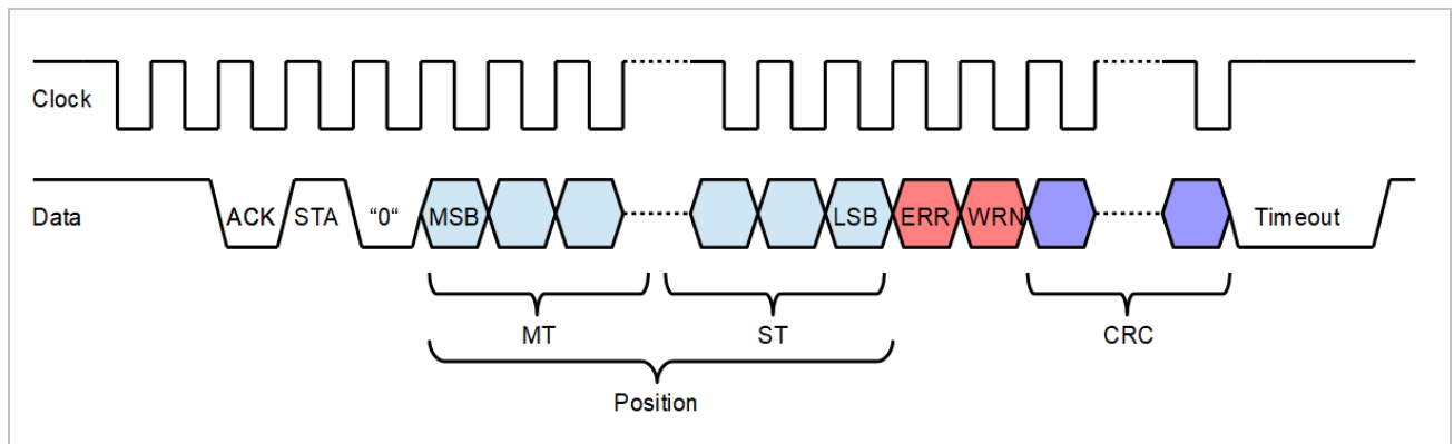
Figure 71: Structure data word BiSS
