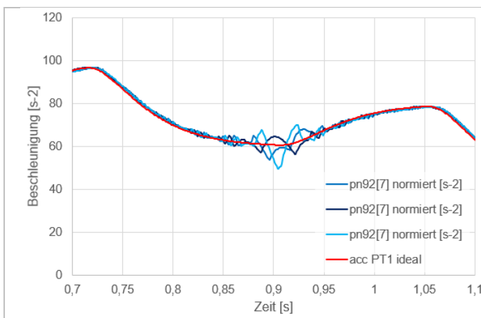
Figure 23: Ripple of the acceleration calculation at small number of increments per revolution
