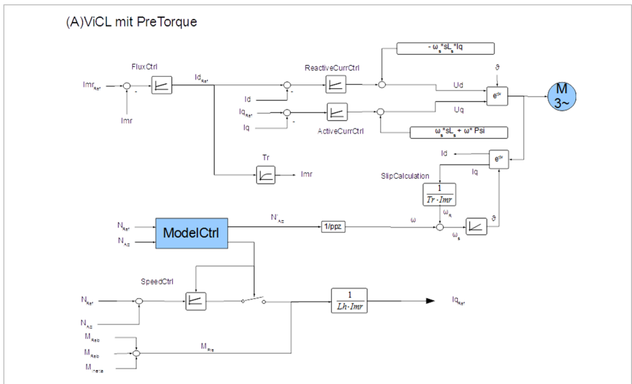
Figure 102: Model deactivation depending on the motor type
