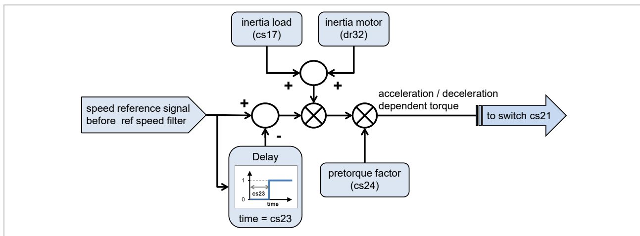
Figure 116: Torque precontrol mode 1
