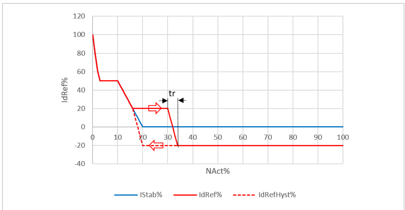
Figure 31: Minimum current course
