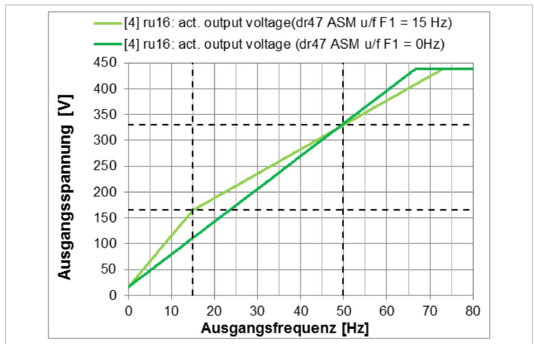
Figure 96: v/f – Influence of the additional setpoint
