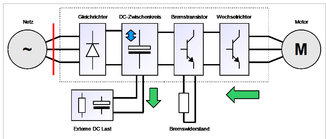
Figure 29: Control to constant DC link voltage
