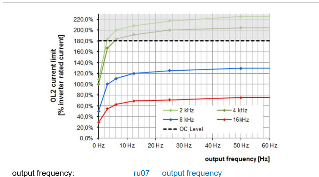
Figure 10: Overload (OL2) limiting characteristic
