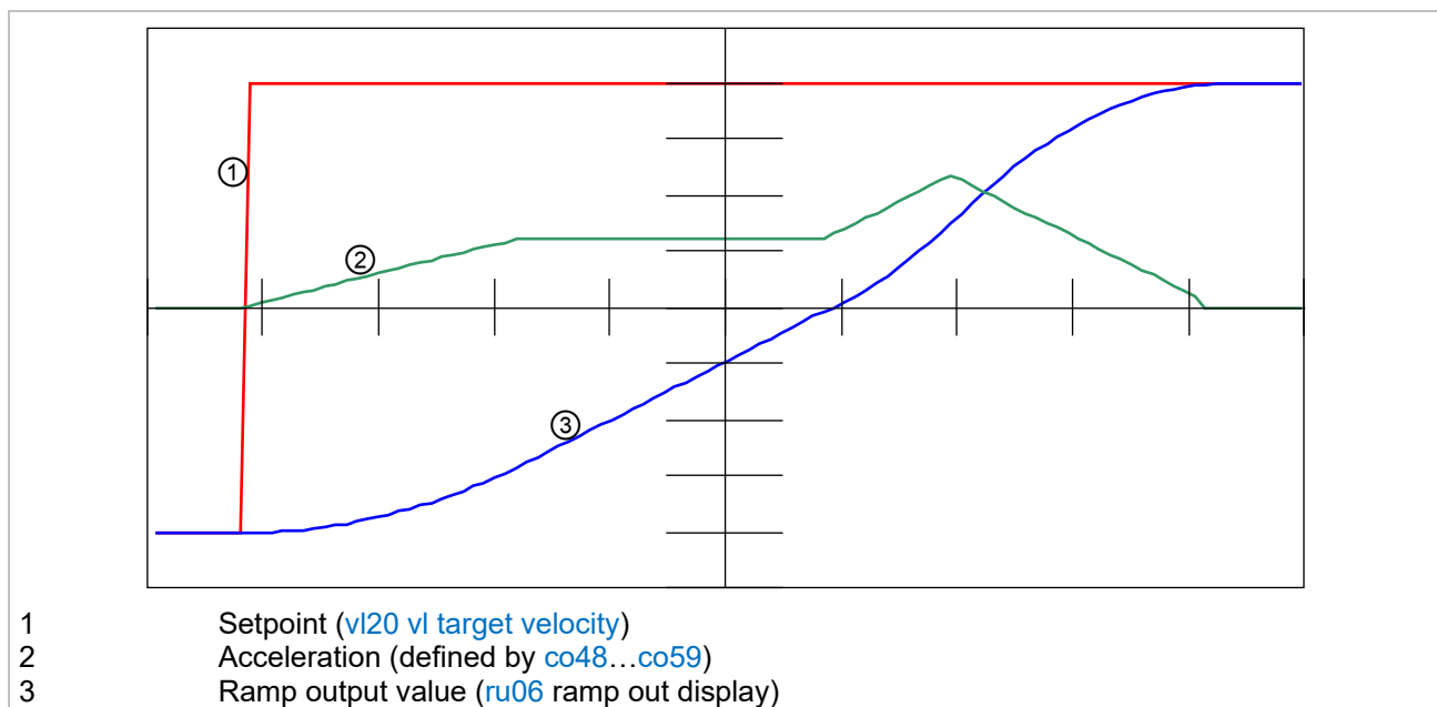
Figure 48: pass zero type = 0: not zero
