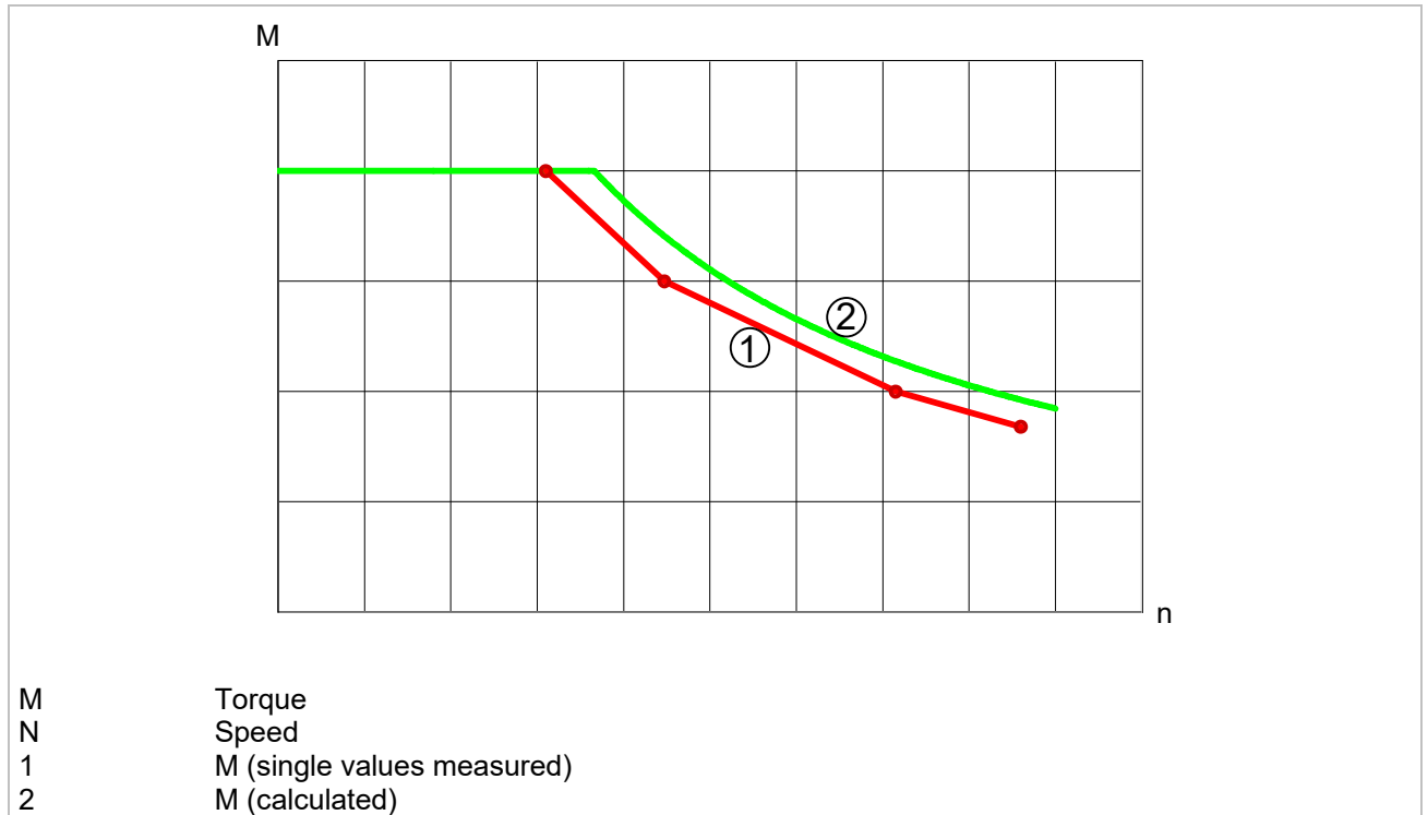
Figure 91: Safety distance to the limit characteristic
