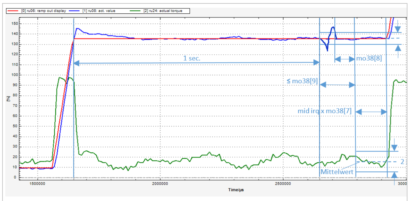
Figure 83: Procedure of the offset measurement
