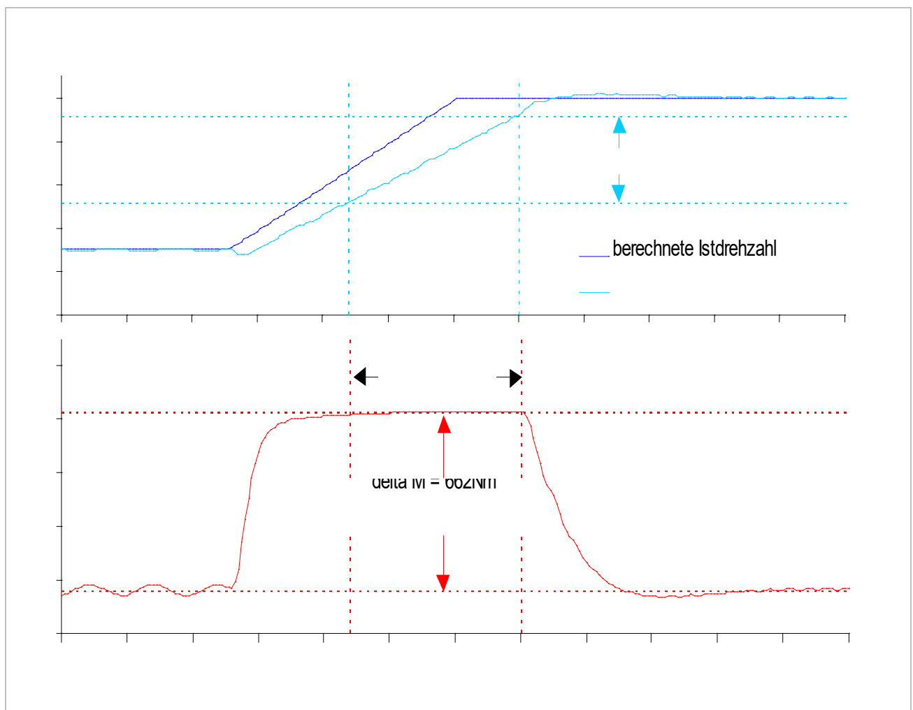
Figure 114: High-run test with COMBIVIS
