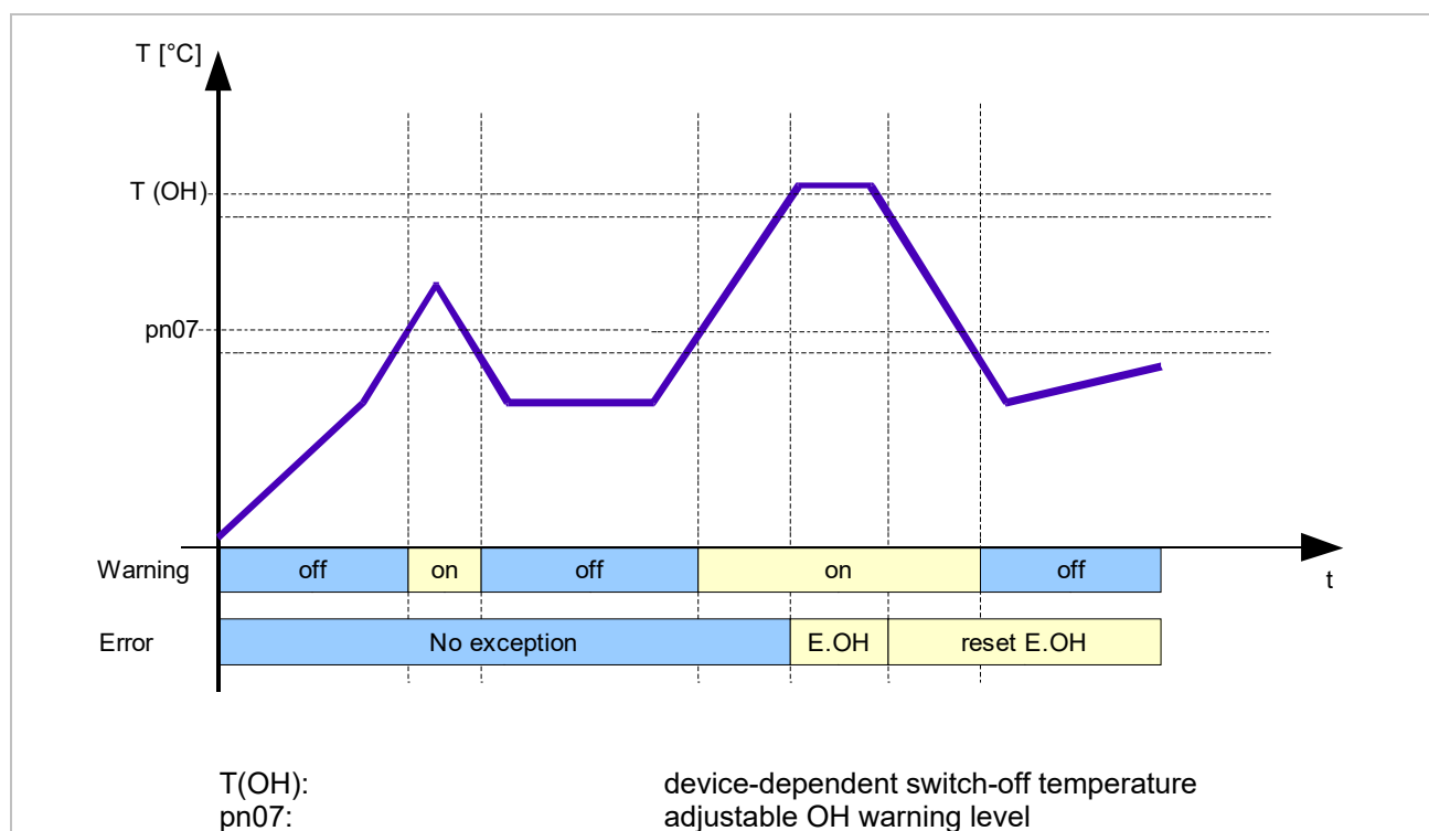
Figure 13: Overtemperature heatsink (OH)
