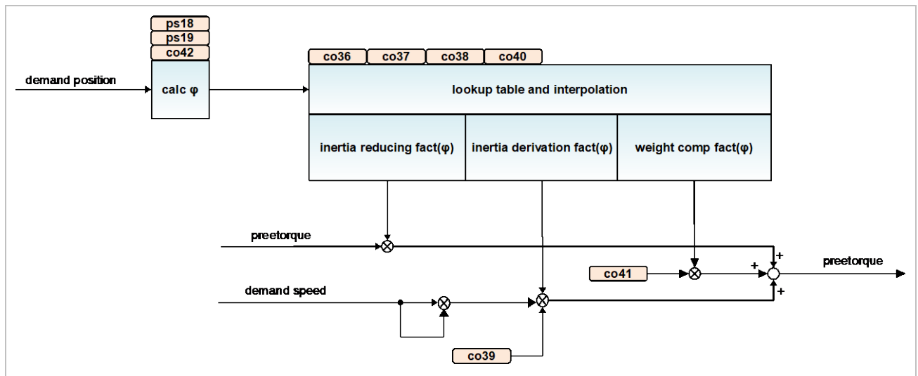
Figure 119: Not linear torque precontrol
