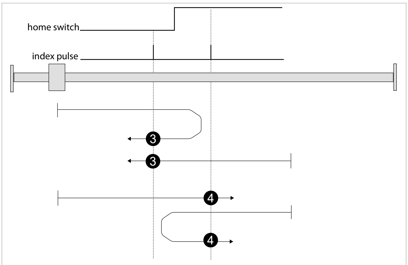
Figure 53: Homing – Method 3 and 4
