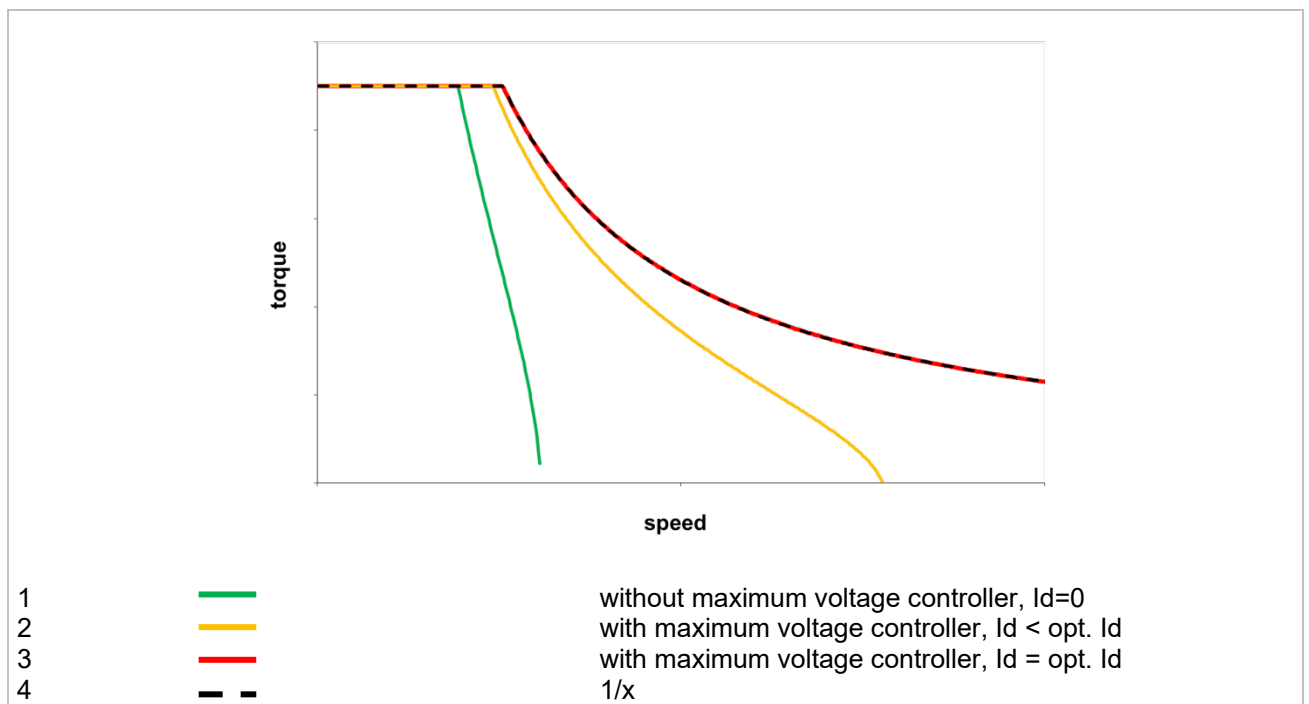
Figure 87: Limit value at synchronous motors
