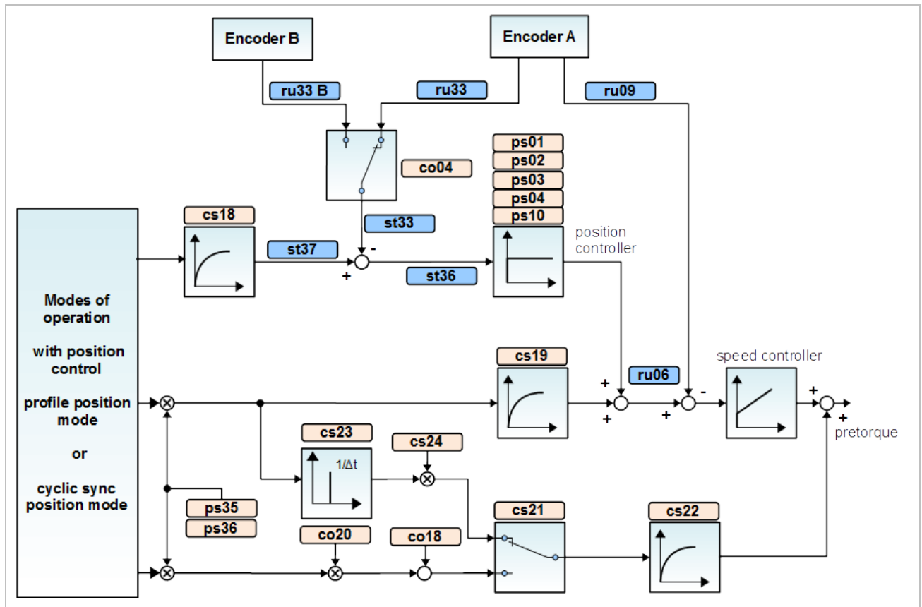
Figure 126: Structure position / speed control
