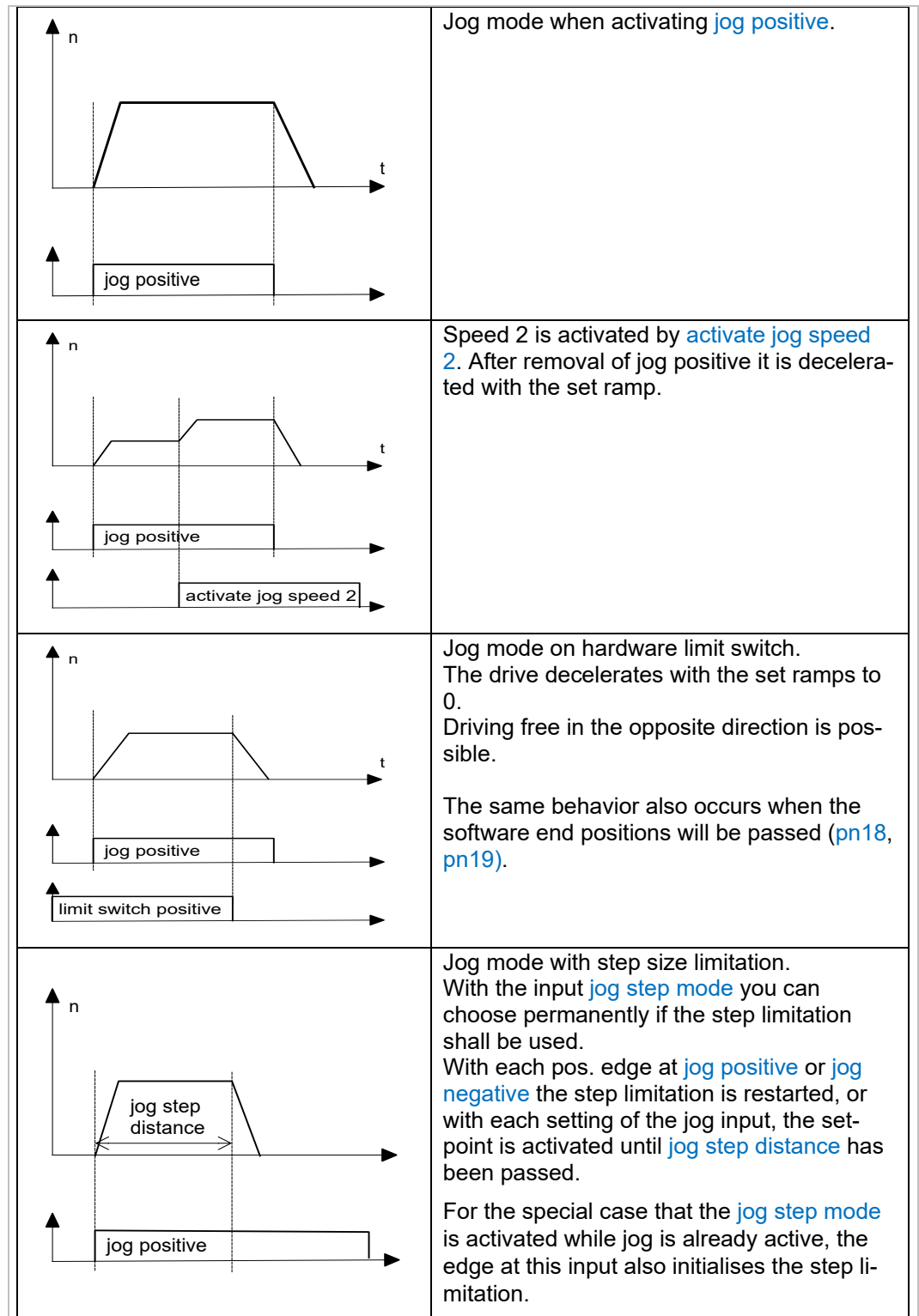
Figure 67: Drive profiles in jog mode
