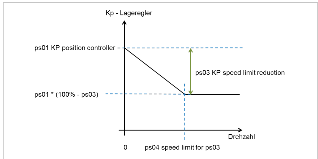
Figure 125: KP reduction in the position controller
