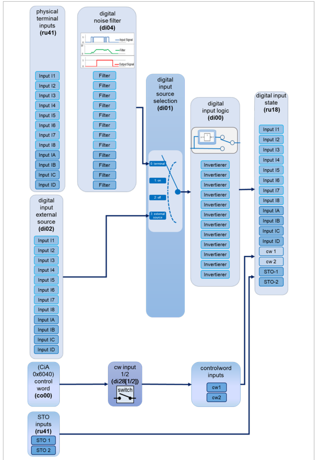
Figure 132: Structure: Evaluation of the digital input status
