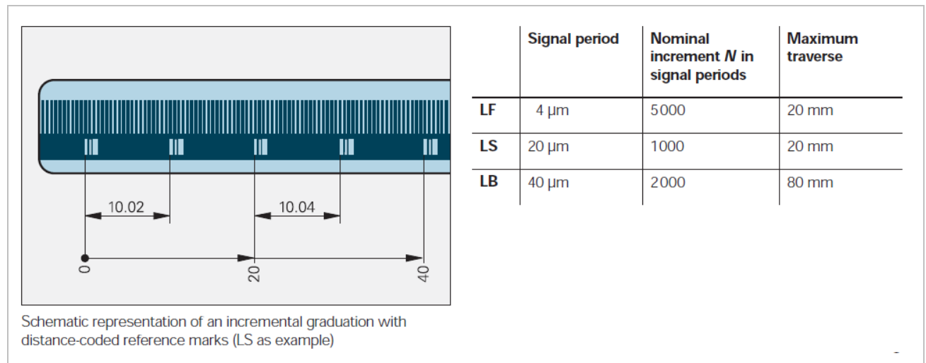
Figure 72: distance-coded reference marks for linear measuring devices from Heidenhain
