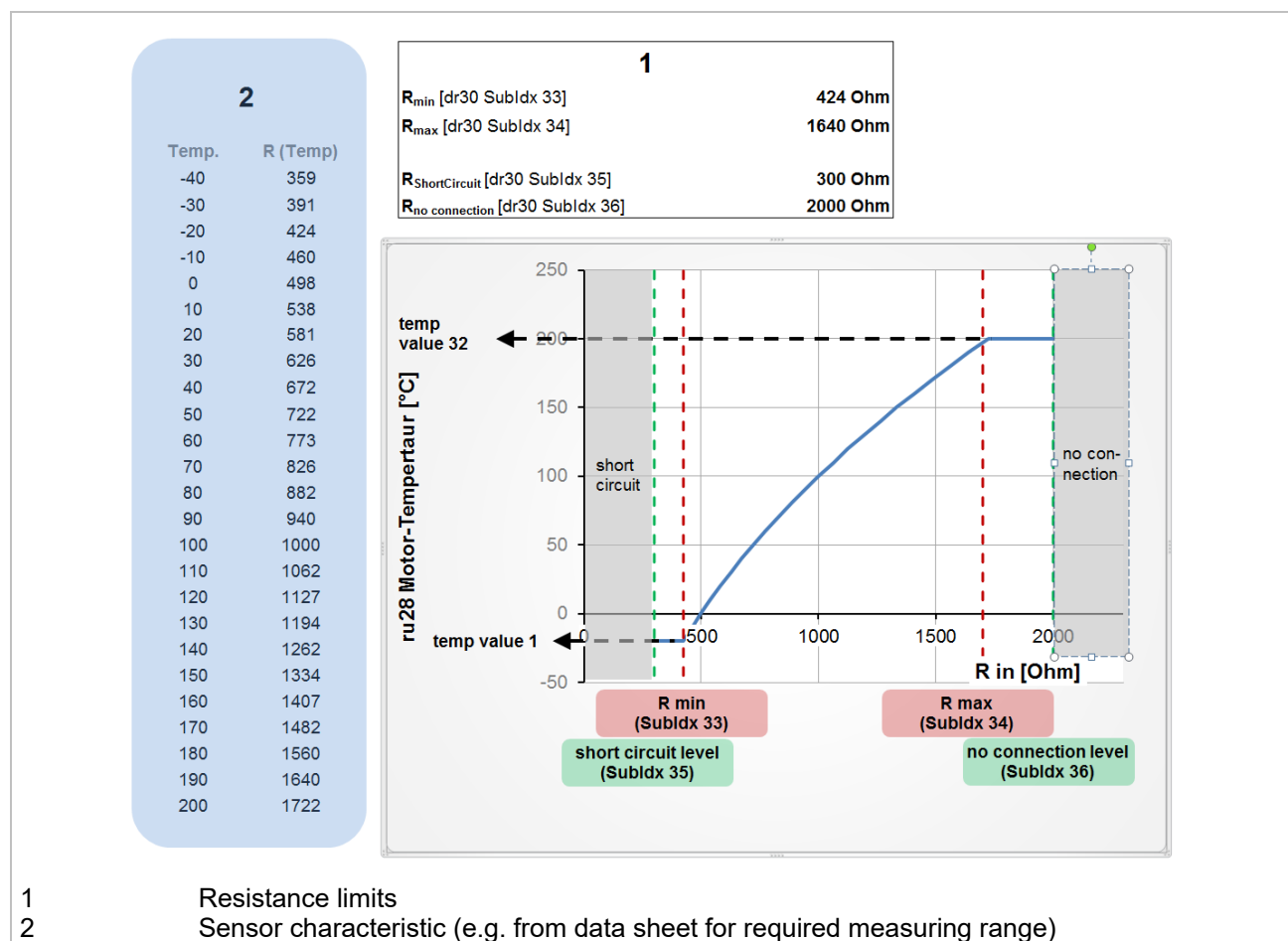
Figure 15: Sensor calculation by Excel
