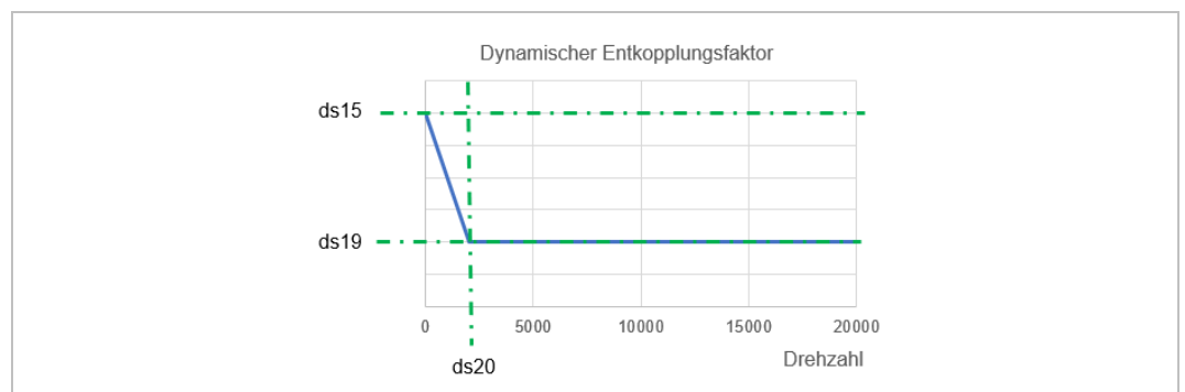
Figure 82: variable dynamic decoupling factor
