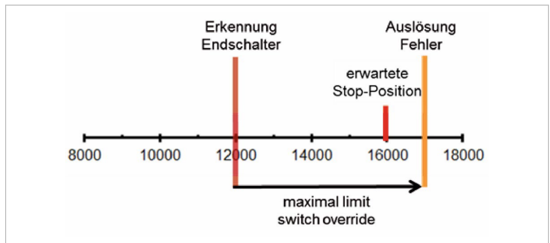
Figure 26: Limit switch
