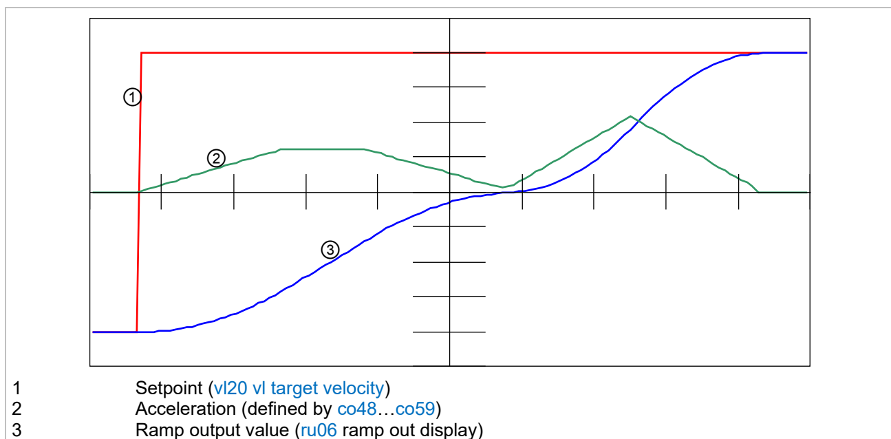
Figure 49: pass zero type = 8: zero
