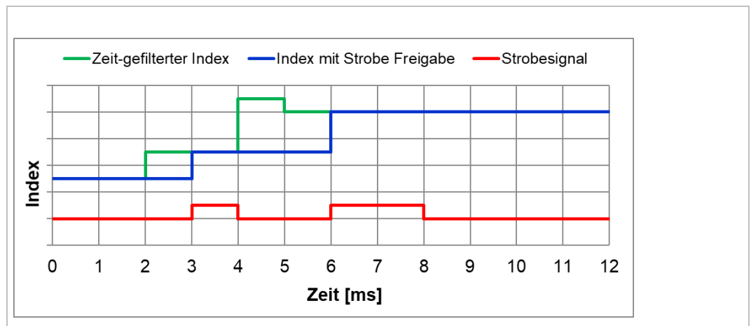
Figure 136: Example index generation with edge-active strobe
