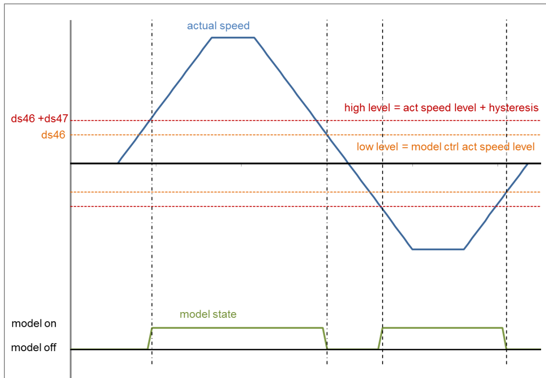
Figure 101: Model deactivation depending on the motor type
