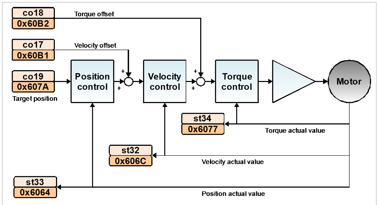
Figure 57: Cyclic synchronous position mode - overview
