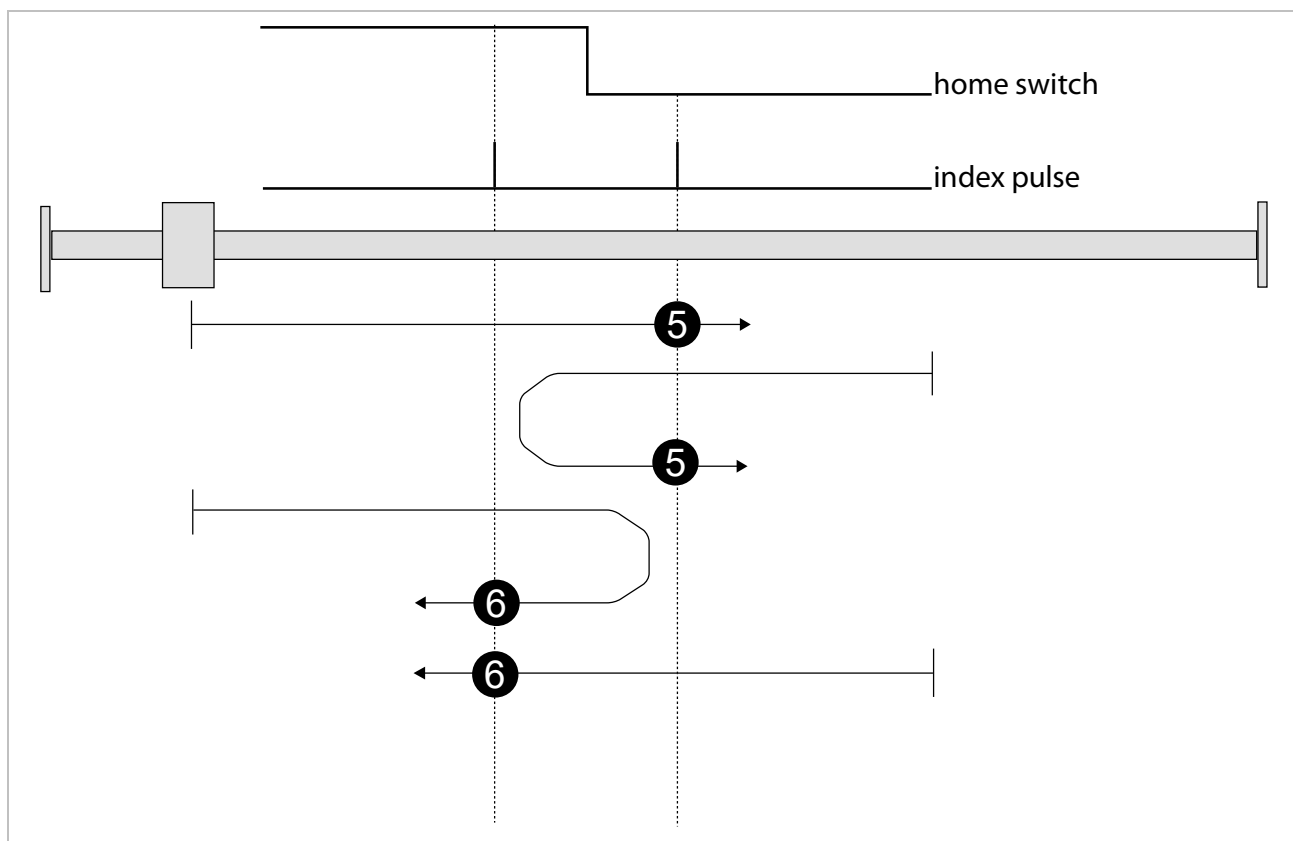
Figure 54: Homing – Method 5 and 6
