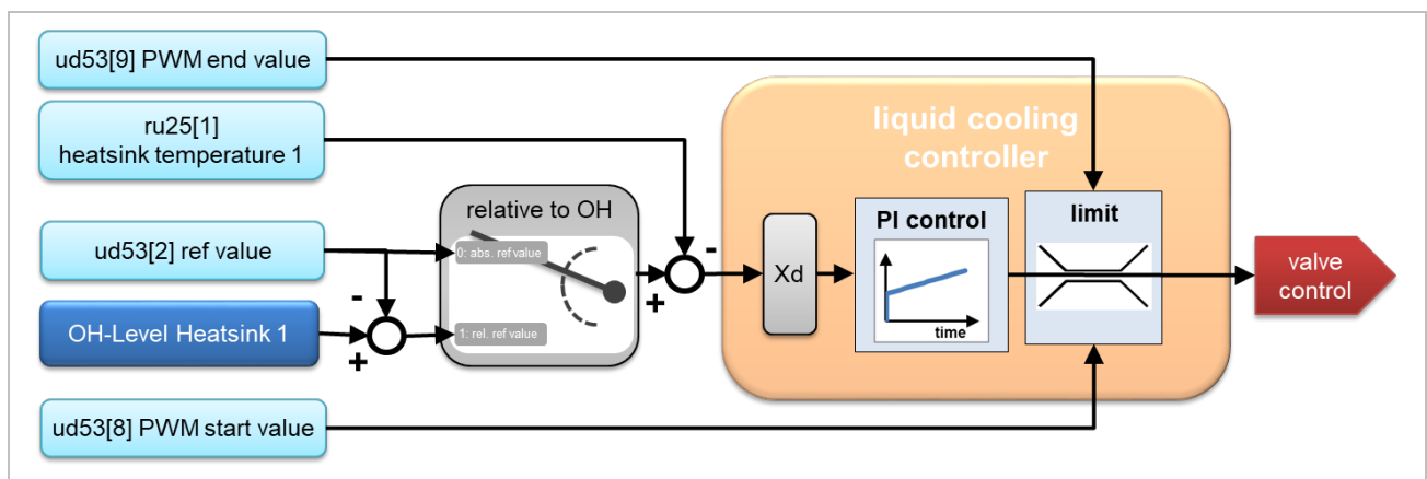
Figure 154: Overview controller
