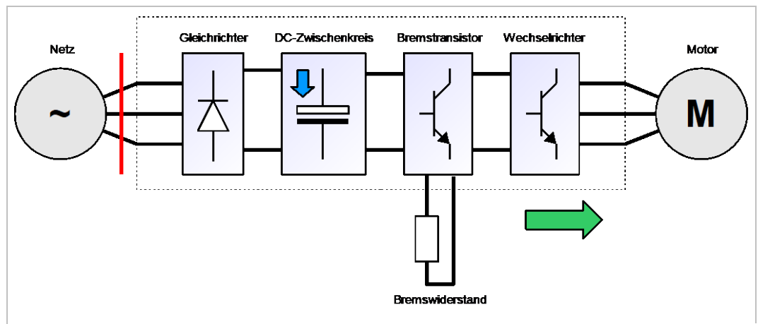
Figure 27: Motor operation without power-off function
