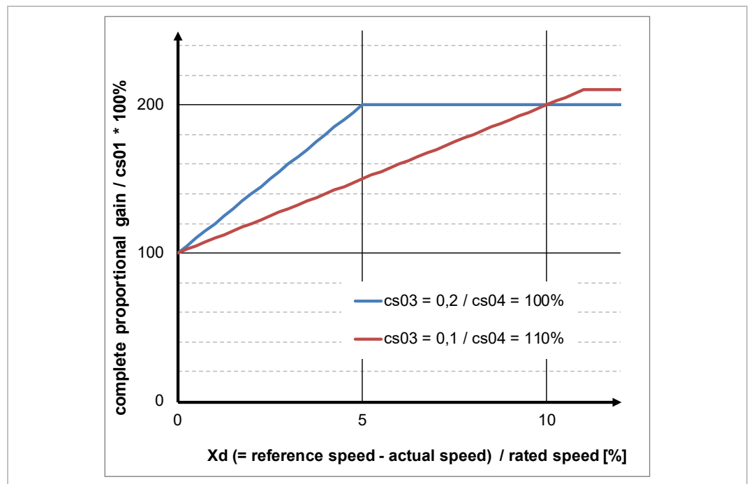
Figure 112: Variable proportional factor
