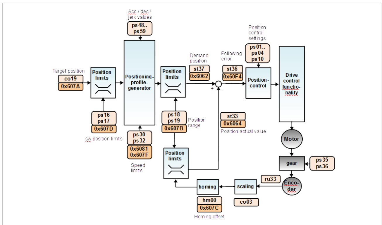
Figure 34: Profile positioning mode (2)
