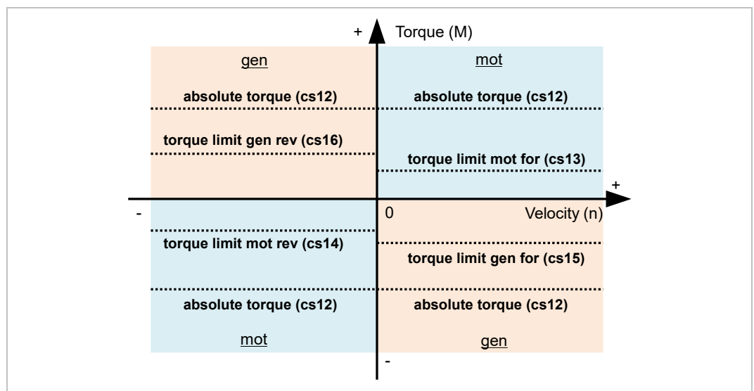
Figure 68: Torque limit in all quadrants
