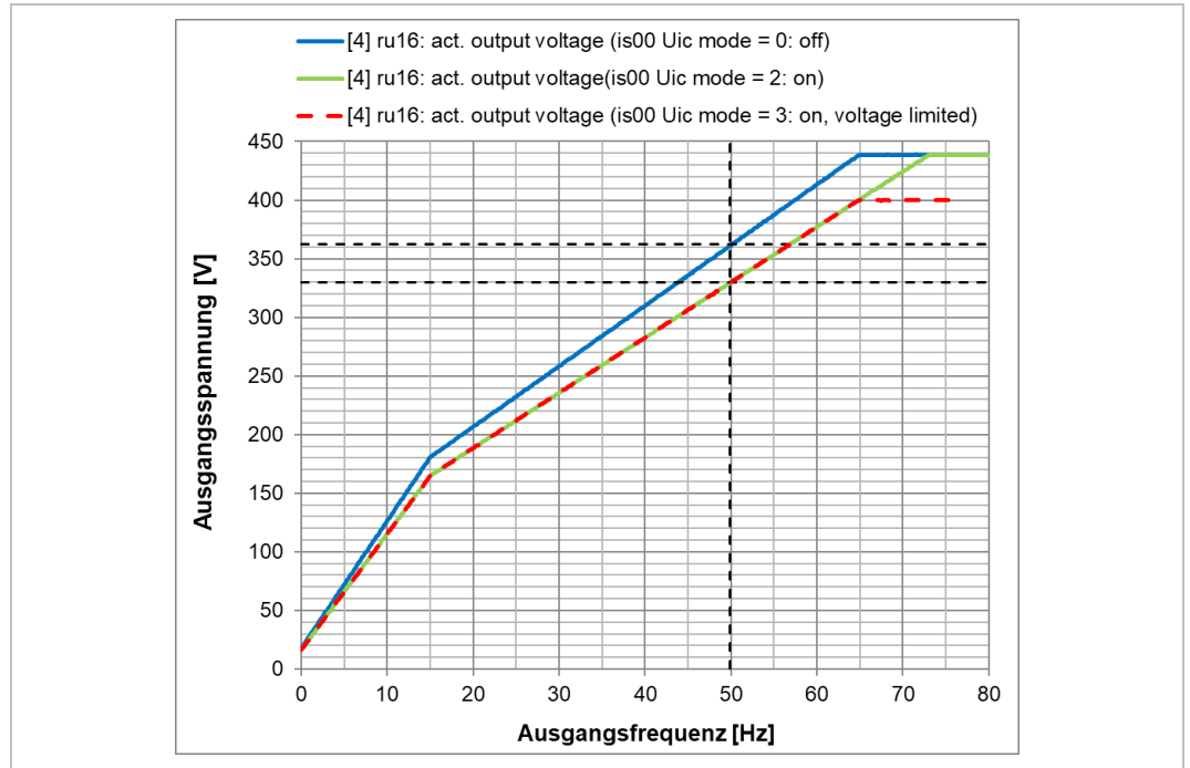
Figure 97: v/f – Influence of the DC link voltage compensation
