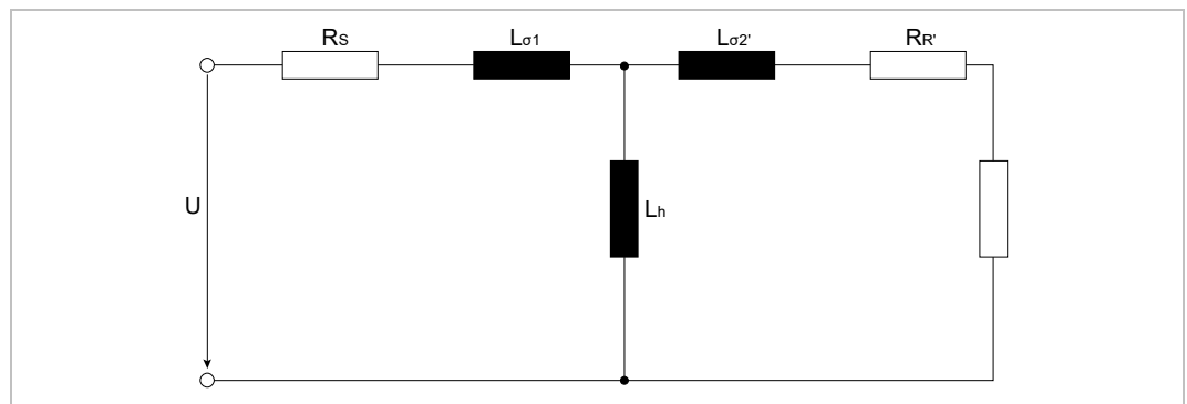
Figure 77: Motor equivalent circuit diagram
