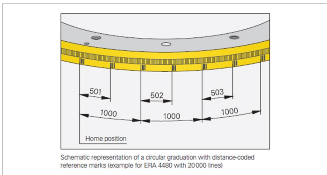
Figure 74: Distance-coded reference marks for rotary encoders
