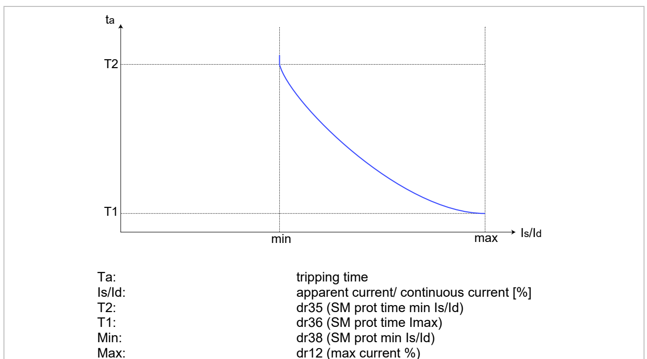
Figure 19: Dependence of the tripping time
