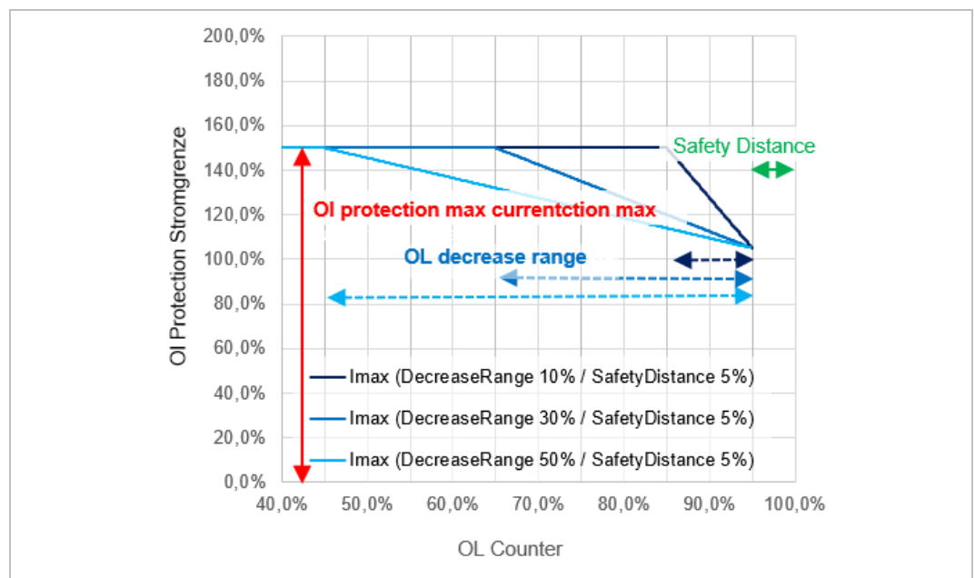
Figure 7: Graph of the current limit depending on the value of the OL counter
