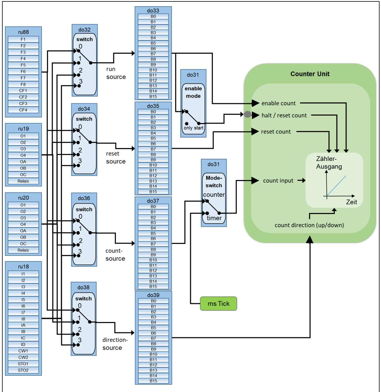
Figure 143: Timer / counter structure
