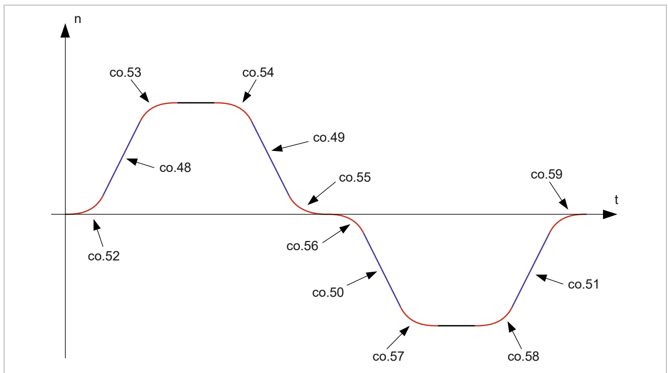
Figure 45: Ramp generator
