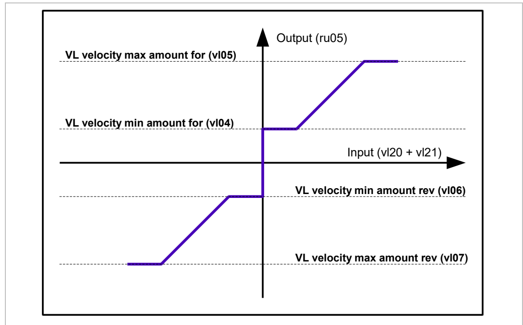
Figure 44: Target speed limitation
