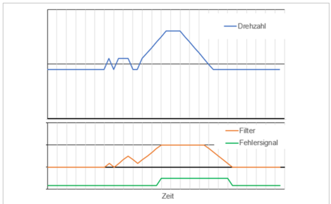
Figure 25: [Filtering of the error signal]
