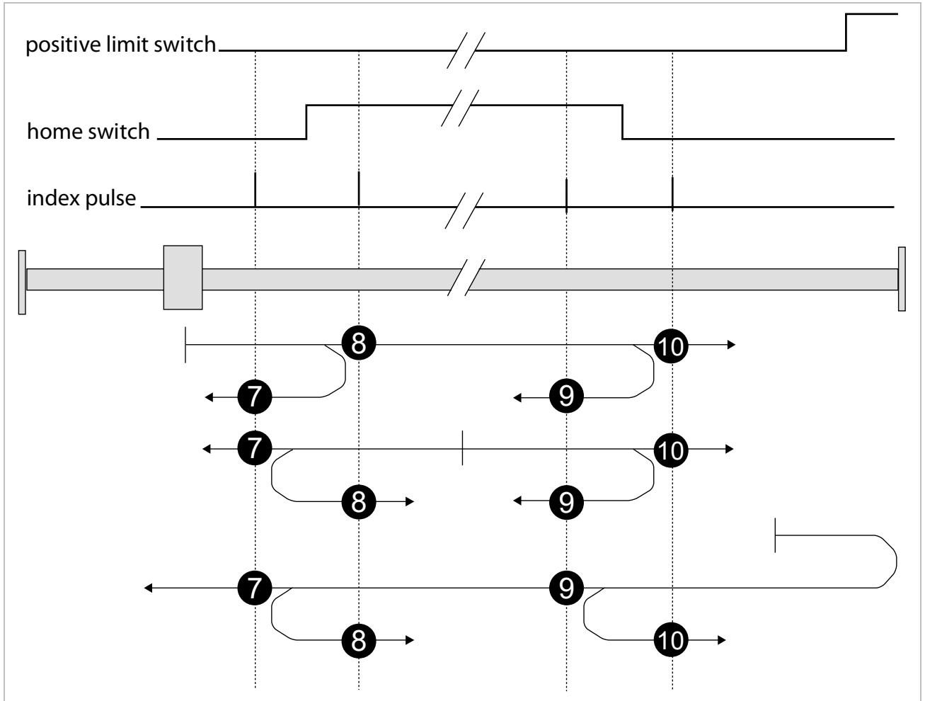
Figure 55: Homing – Method 7 to 14 (23 to 26)
