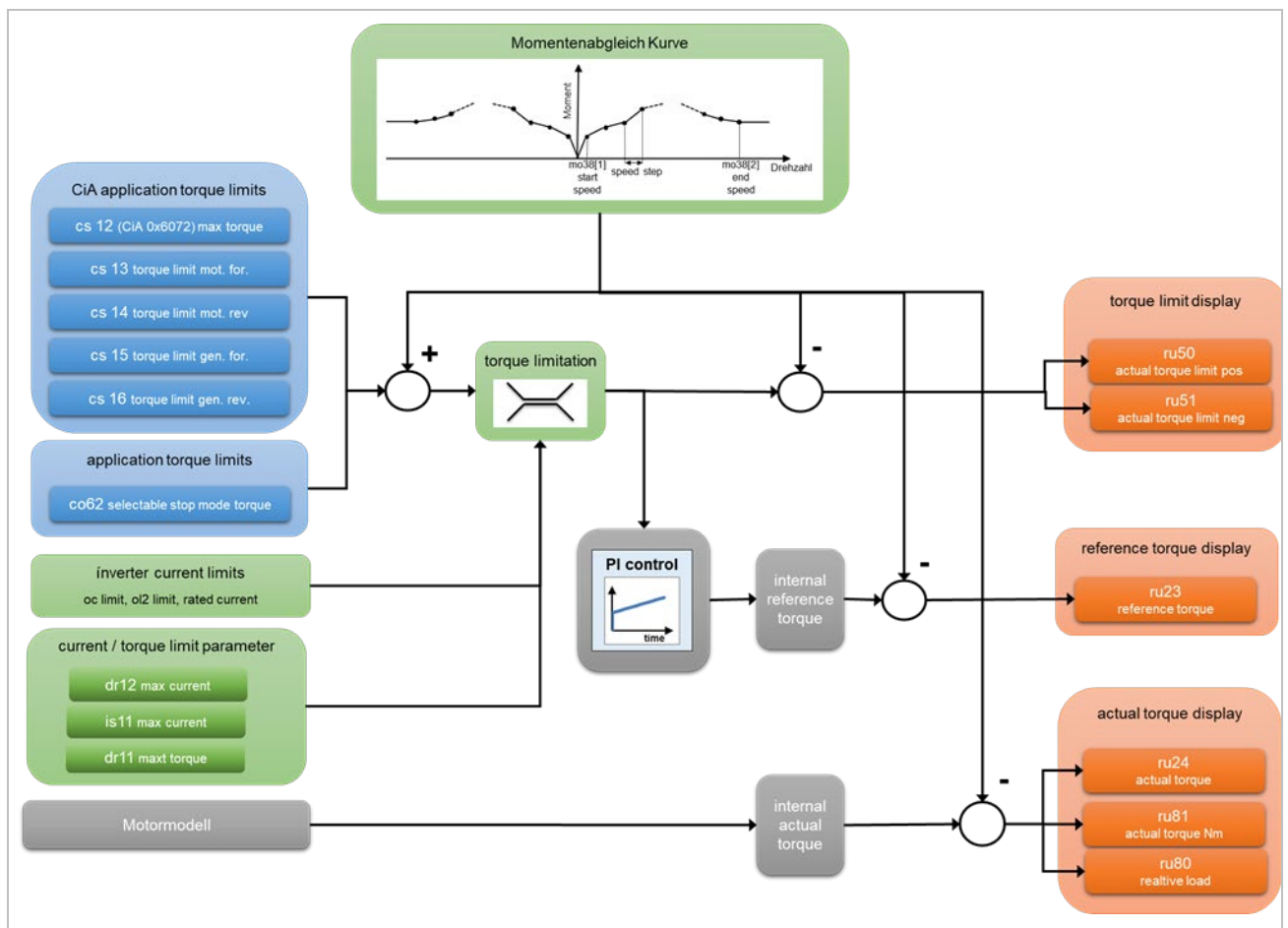
Figure 84: simplified representation of the torque offset compensation
