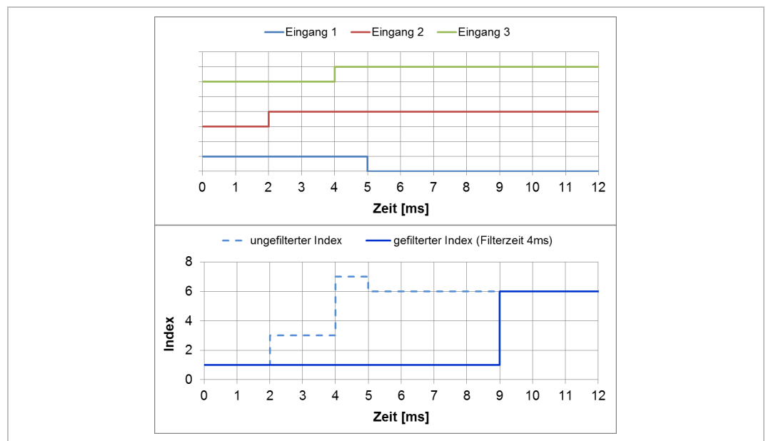
Figure 135: Example for the index filter
