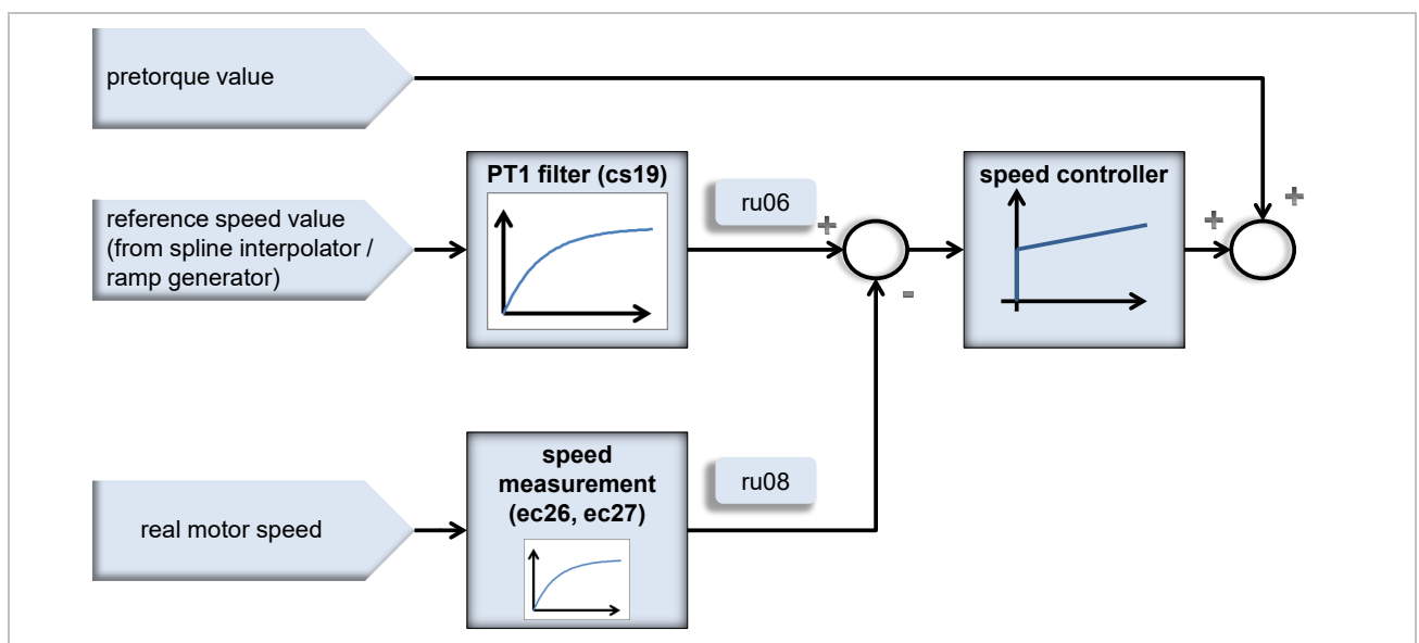
Figure 121: Speed setpoint deceleration
