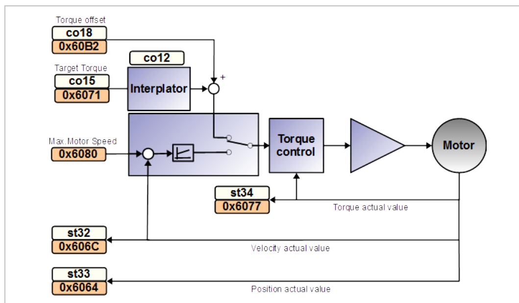
Figure 63: Cyclic synchronous torque mode - Overview
