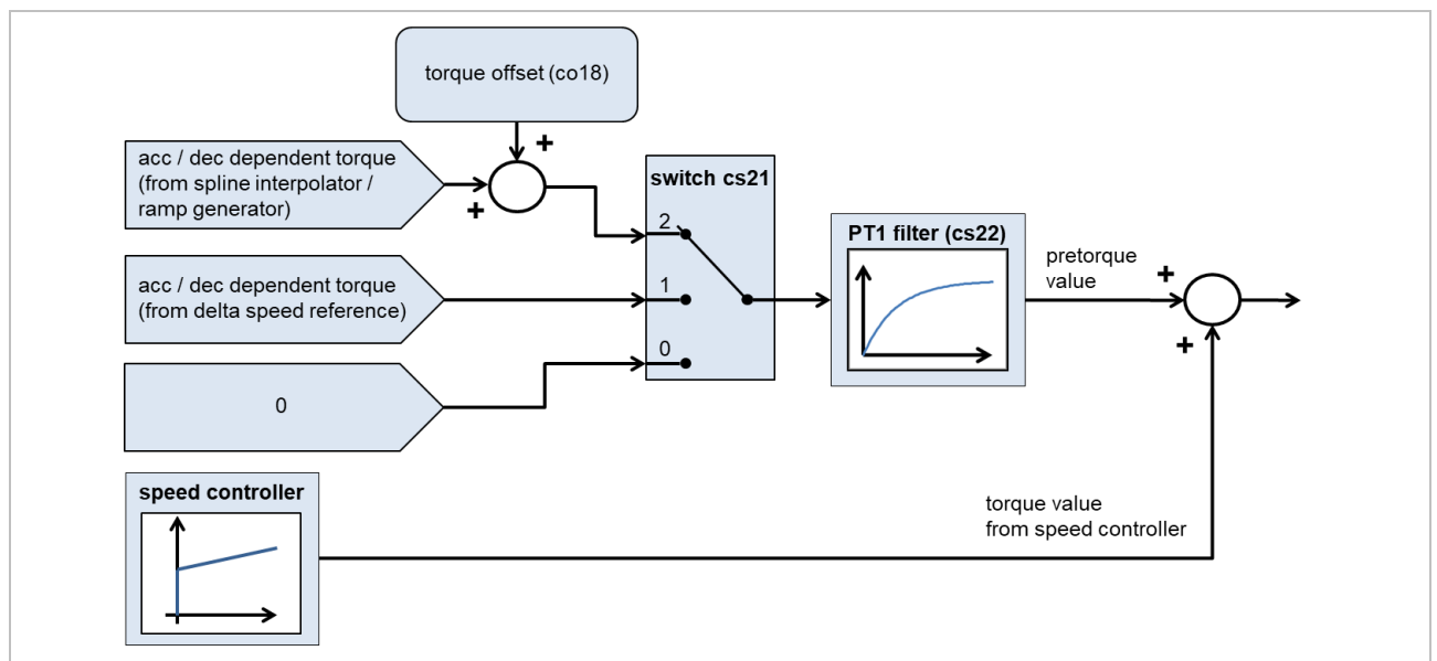
Figure 118: Torque precontrol smoothing
