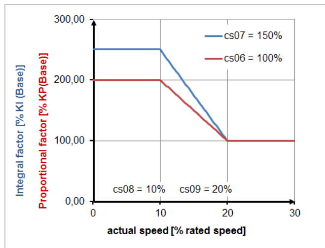
Figure 113: Variable proportional factor (kp) / integral factor (ki) with cs08=10%, cs09=20%
