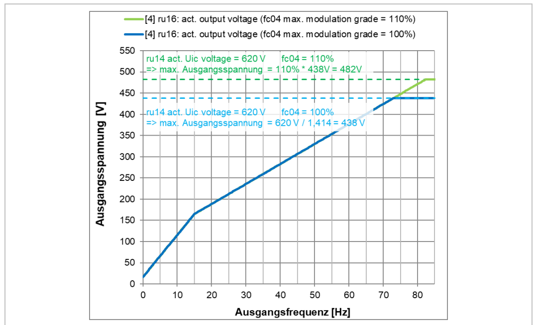
Figure 98: v/f – Influence of the maximum modulation grade
