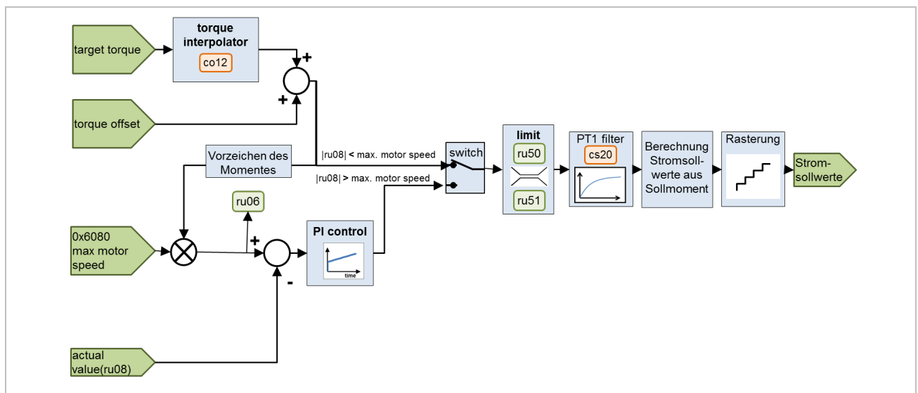
Figure 65: Torque control and overspeed interception
