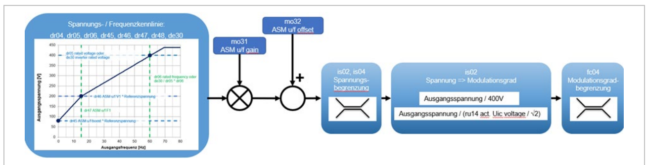
Figure 95: [Sequence modulation factor calculation]
