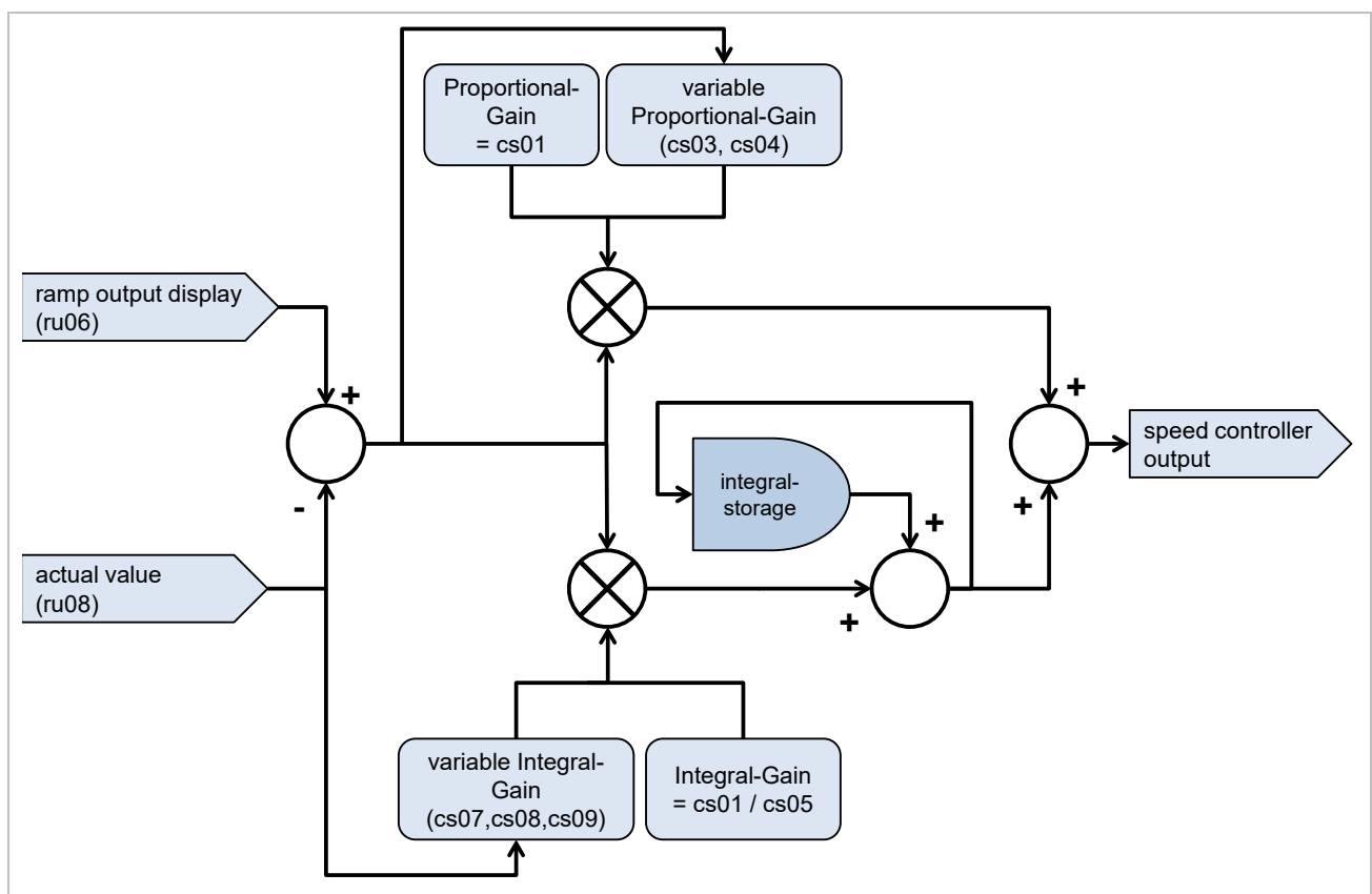
Figure 111: Pi-speed controller
