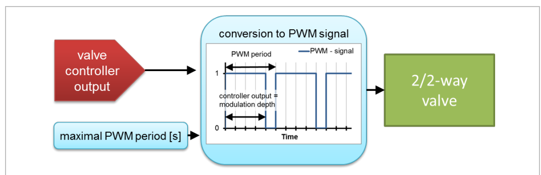
Figure 156: Structure PWM for cooling control
