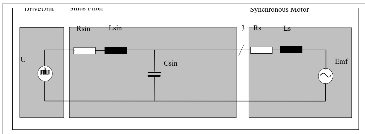
Figure 108: Connection example sinus filter
