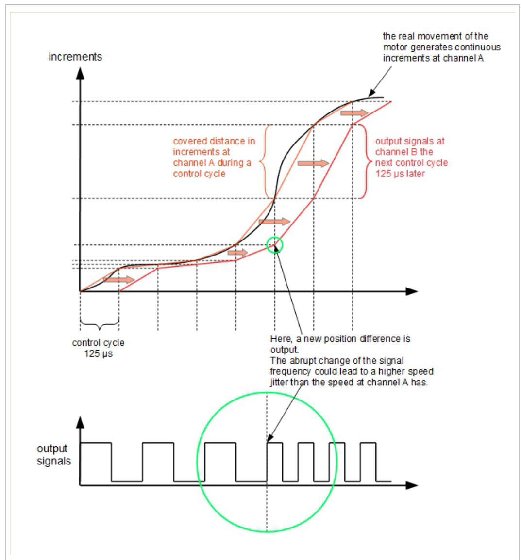
Figure 76: Incremental encoder emulation
