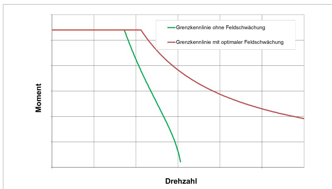
Figure 90: Limit characteristic curve
