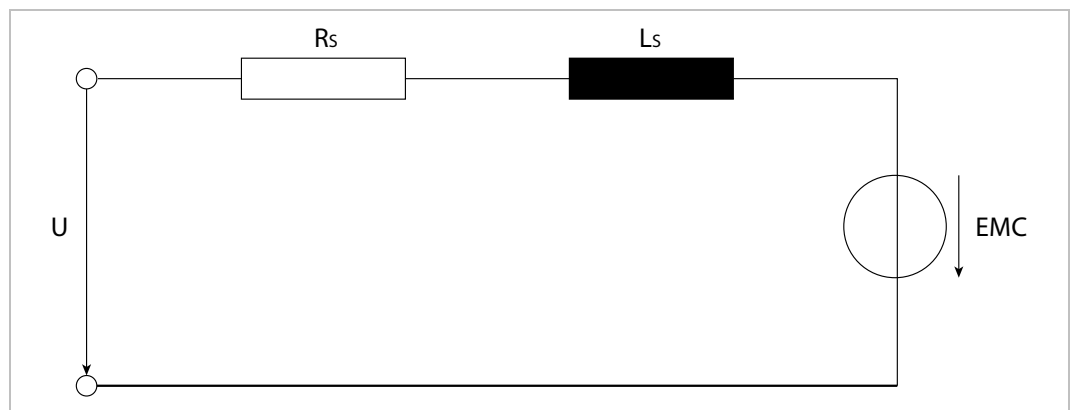
Figure 78: Equivalent circuit diagram synchronous motor
