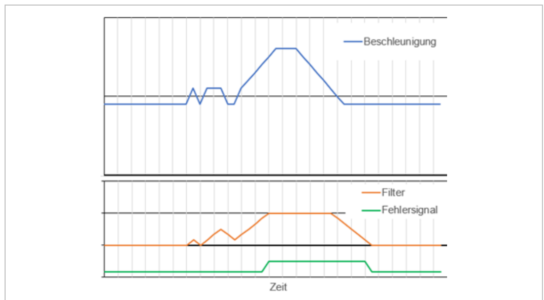
Figure 24: Error signal filter
