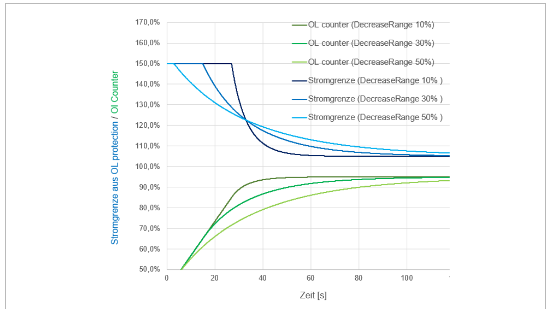
Figure 8: temporal graph of OL counter and current limit
