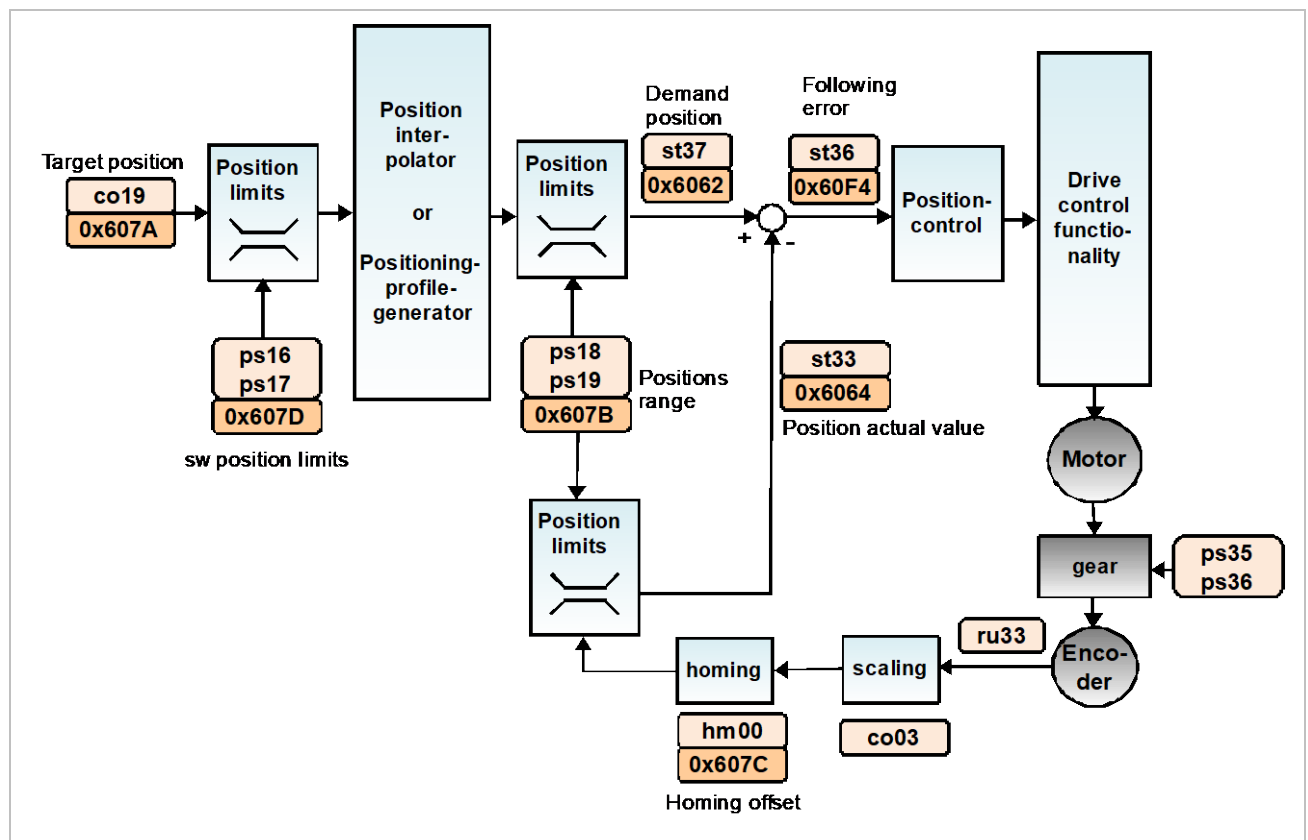
Figure 124: Position control overview
