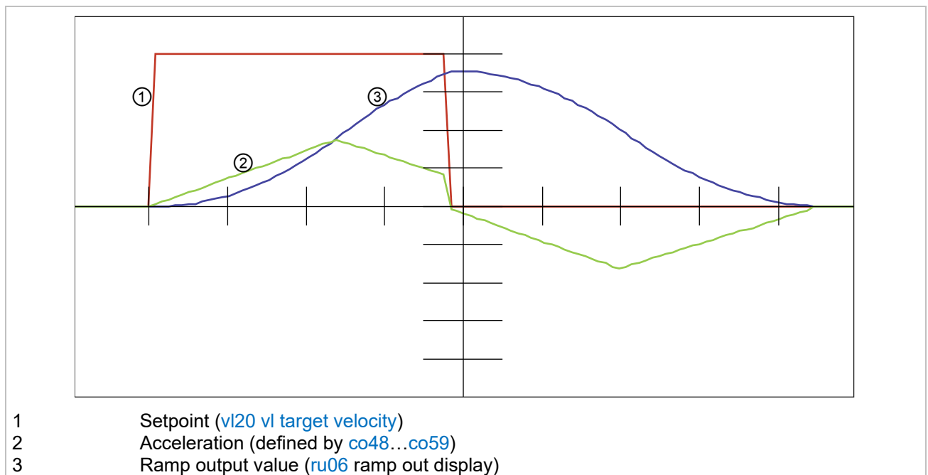
Figure 47: s-curve type = 4: abort in s-curve
