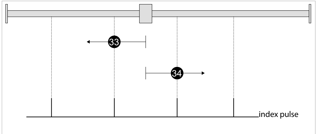
Figure 56: Homing – Method 33 and 34
