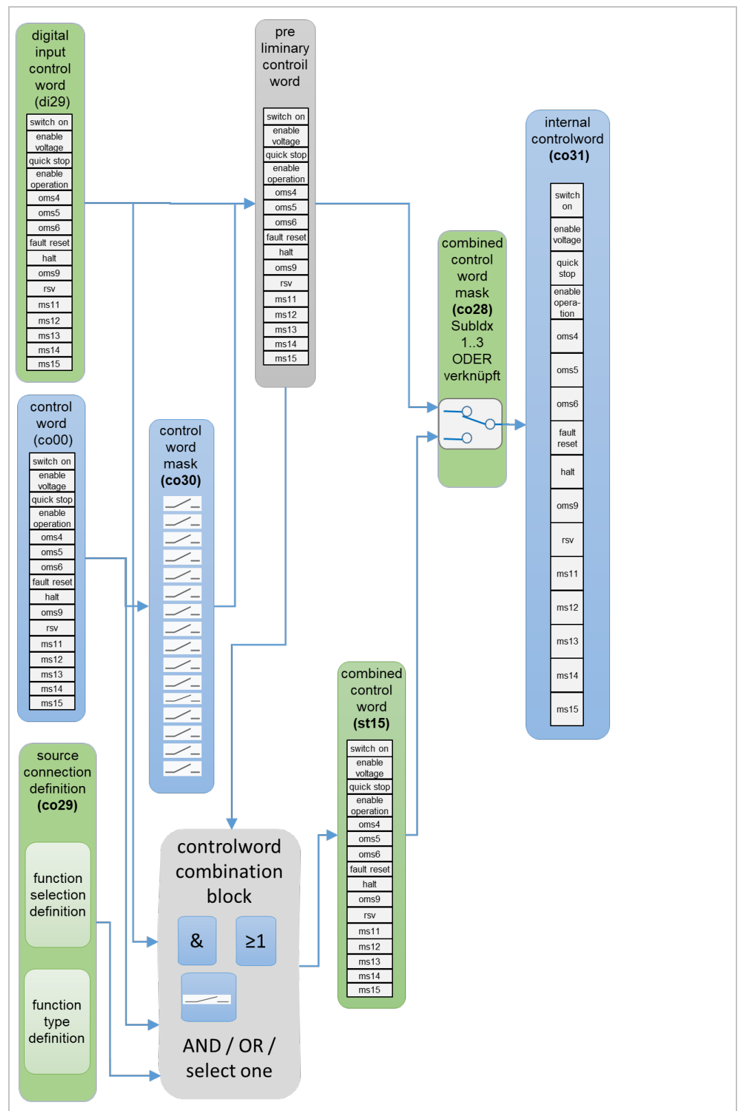
Figure 134: digital input controlword
