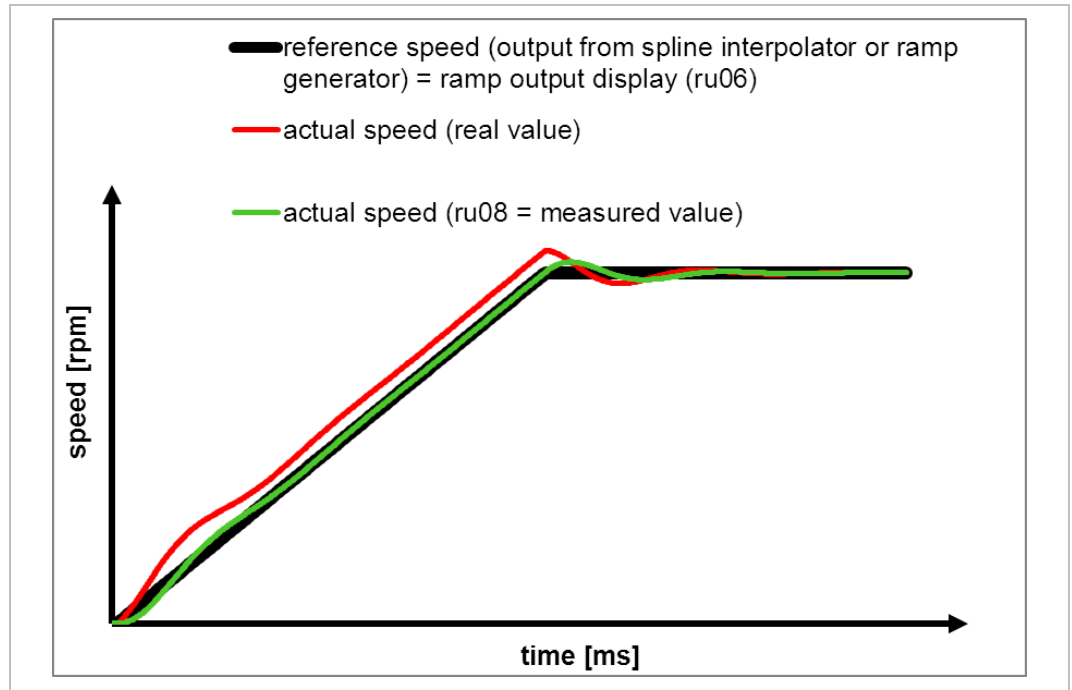
Figure 120: Overshoots in the speed setpoint
