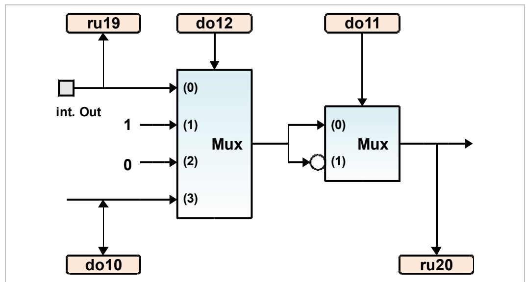
Figure 138: Digital outputs block diagram
