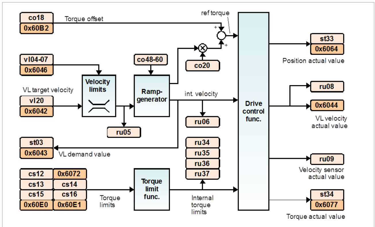
Figure 43: Velocity mode
