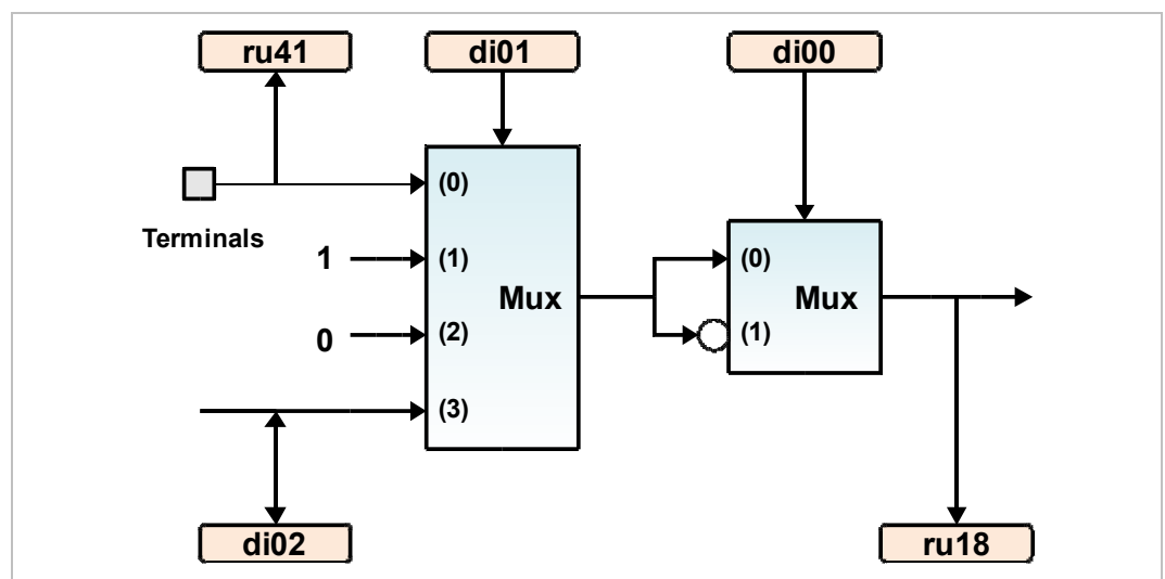
Figure 127: Digital inputs block diagram
