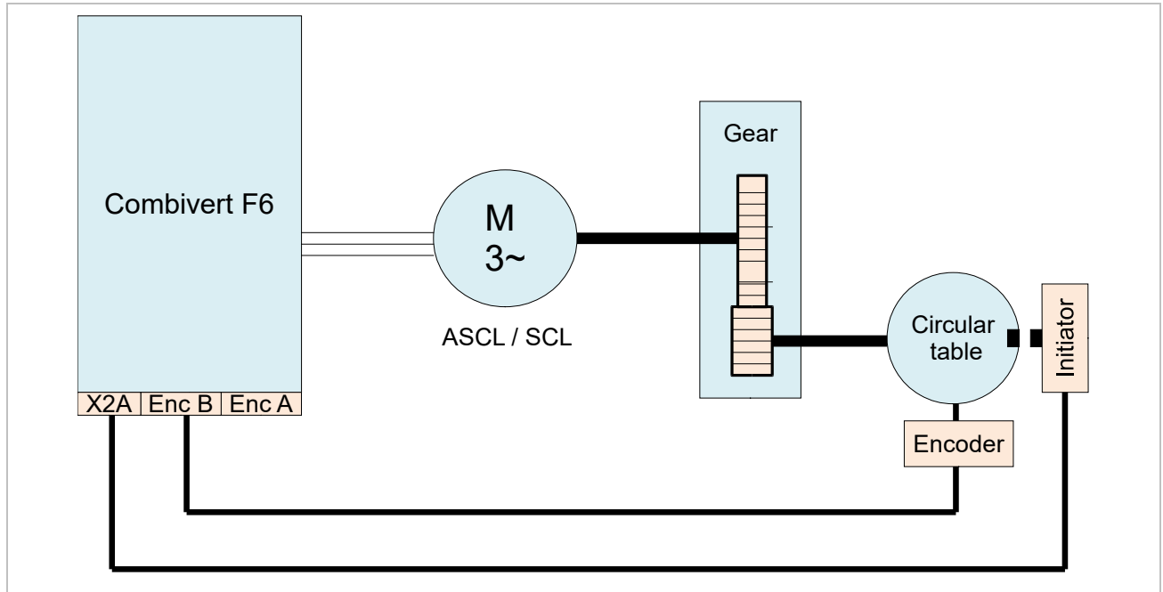
Figure 41: Operation with motor model and encoder with initiator at rotary table
