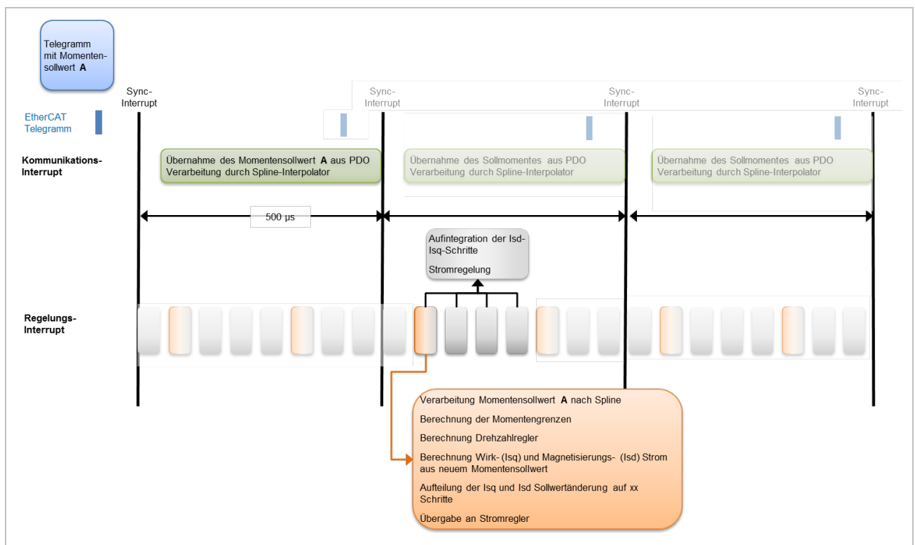
Figure 64: Transfer torque setpoint telegram -> current controller
