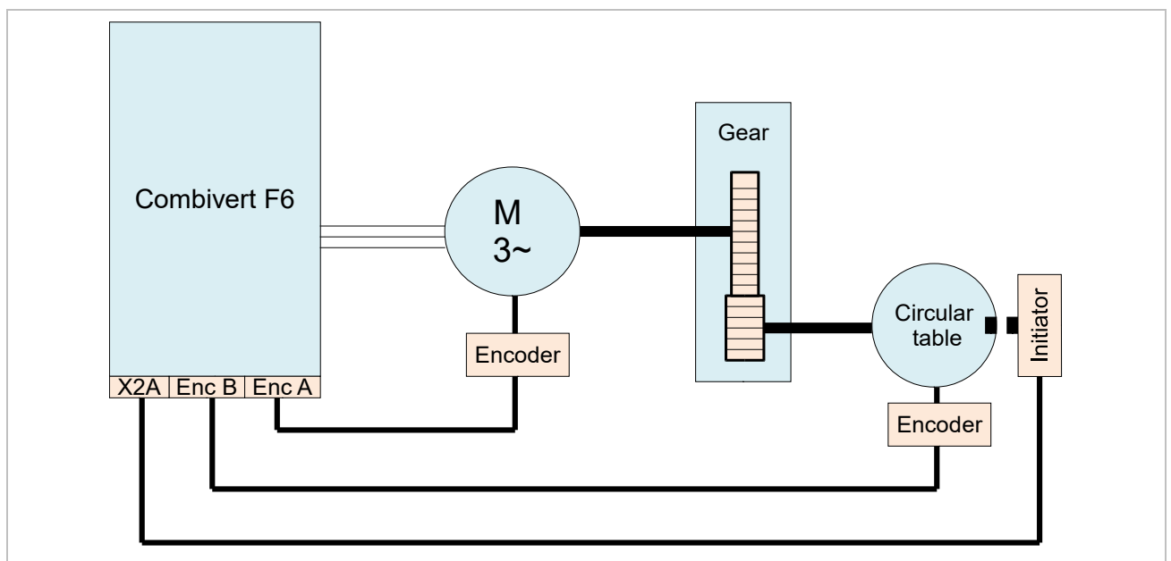
Figure 40: Motor encoder with encoder and initiator at rotary table
