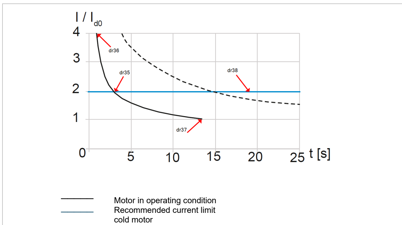
Figure 20: Determination of the motor protection function data from the characteristics of the motor manufacturer
