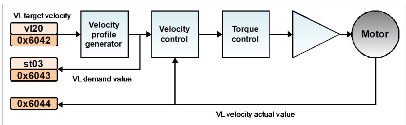
Figure 42: Velocity mode - overview
