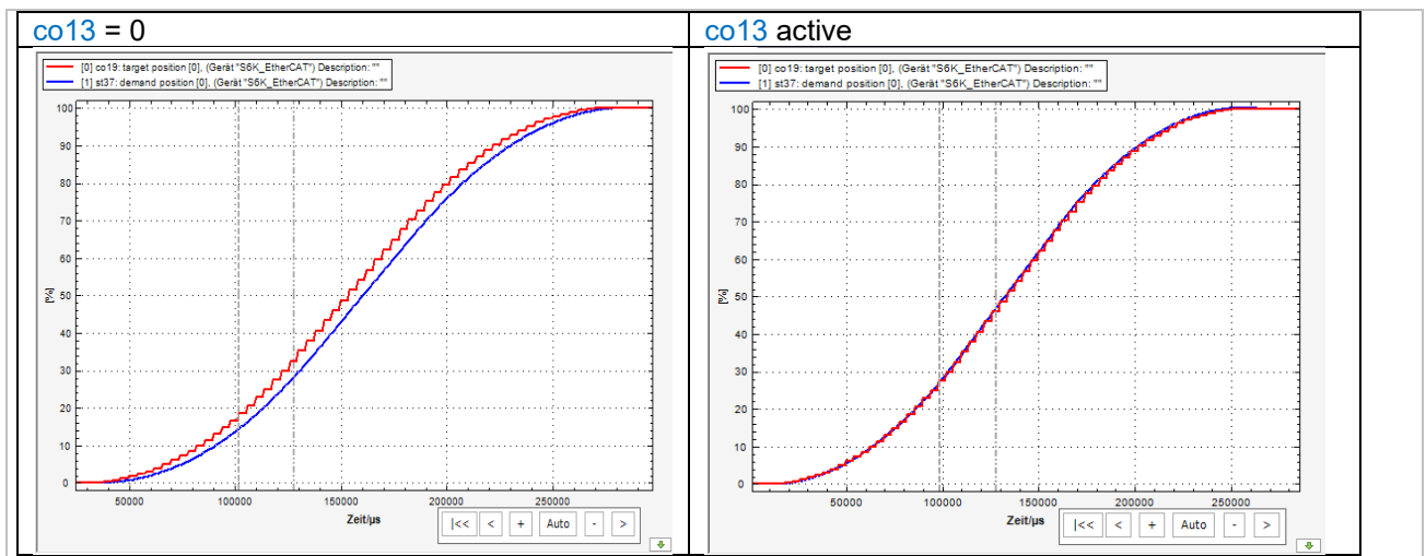
Figure 60: Position precontrol
