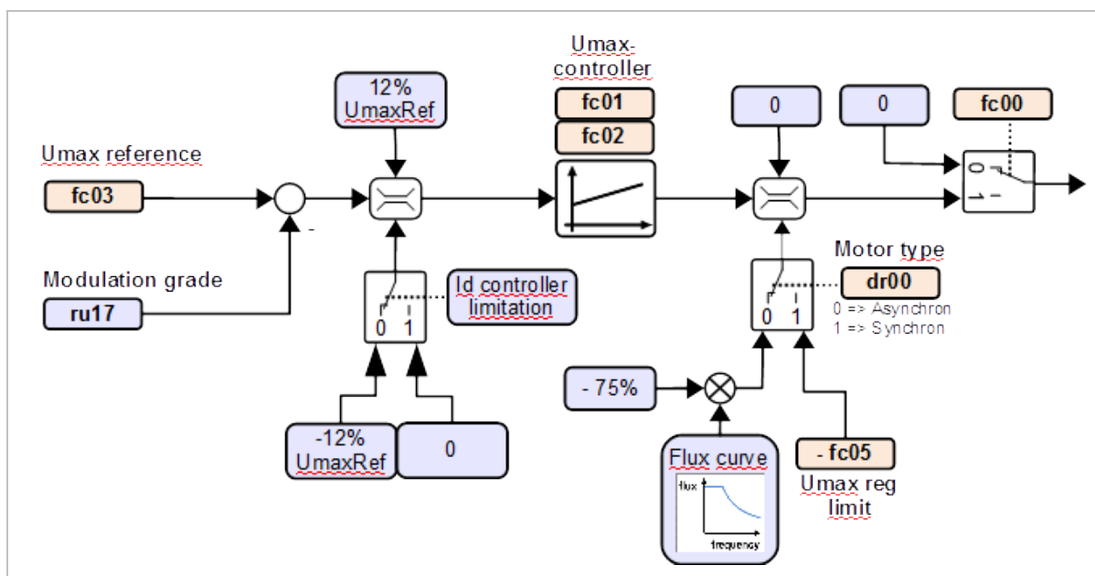
Figure 86: Maximum voltage controller
