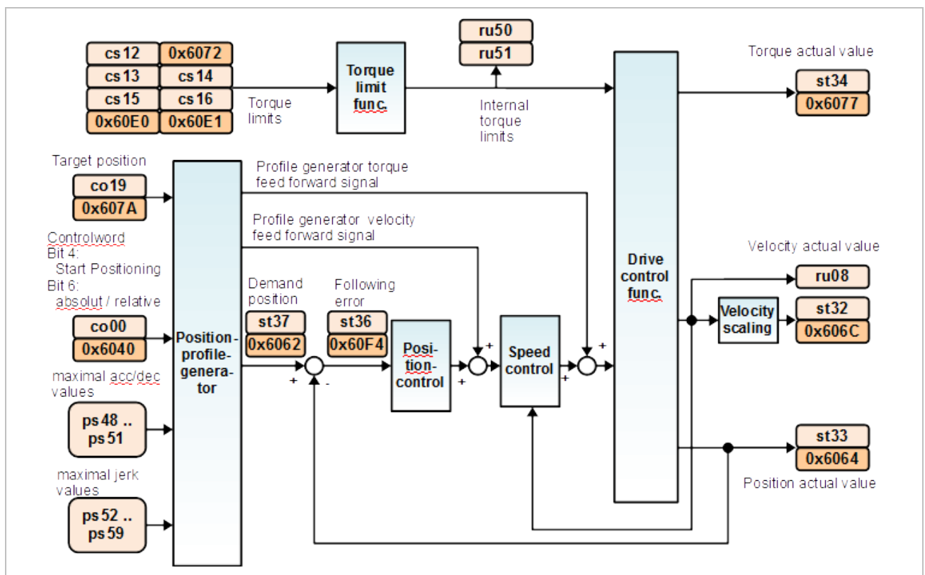
Figure 33: Profile positioning mode (1)
