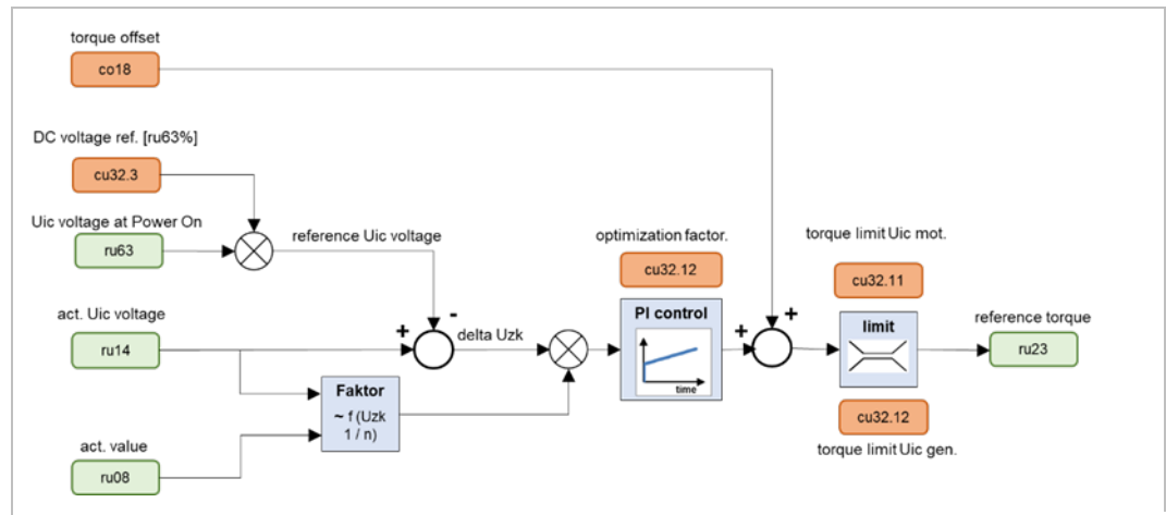
Figure 30: Circuit diagram of the DC control
