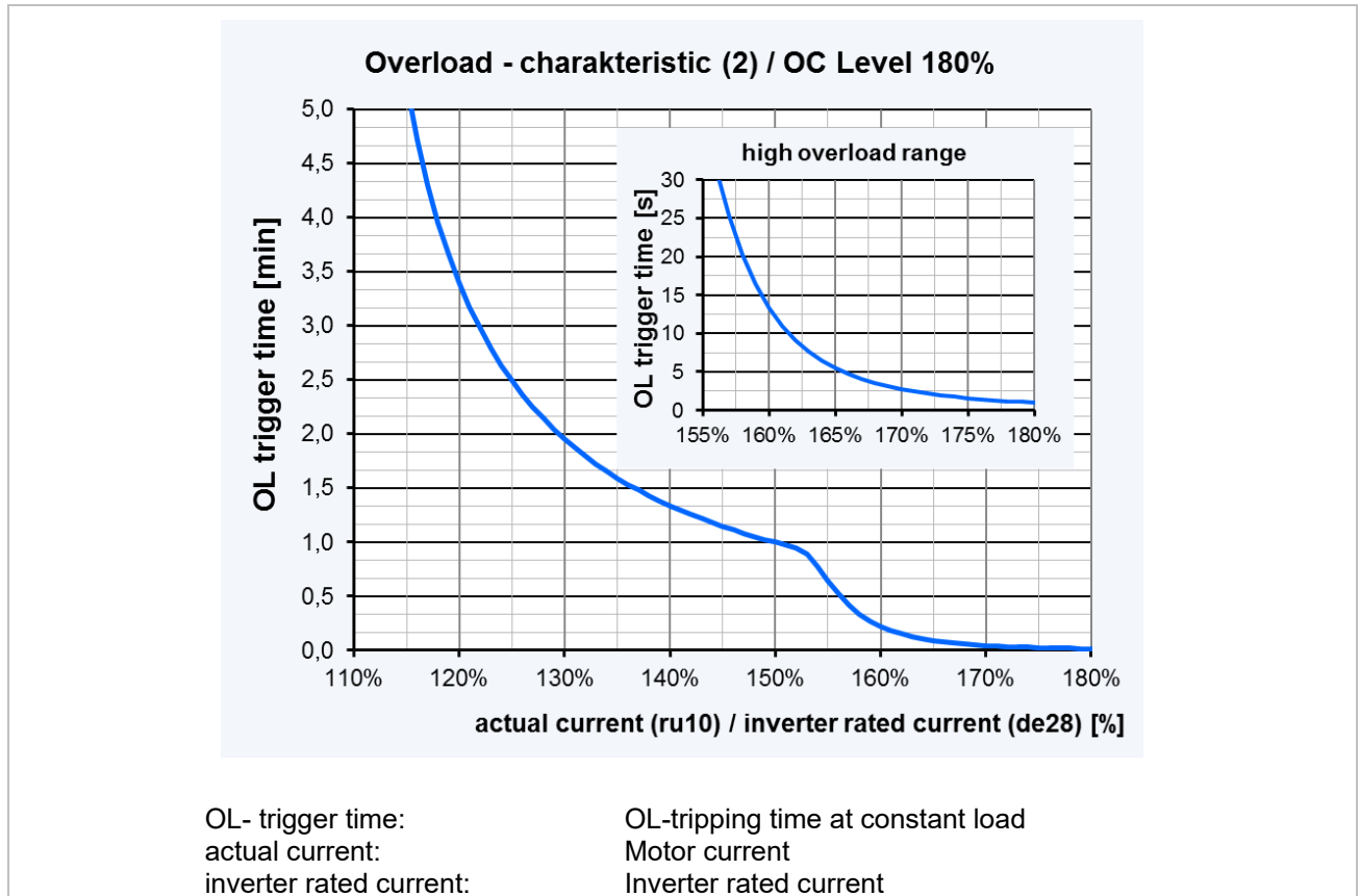
Figure 6: Overload characteristic
