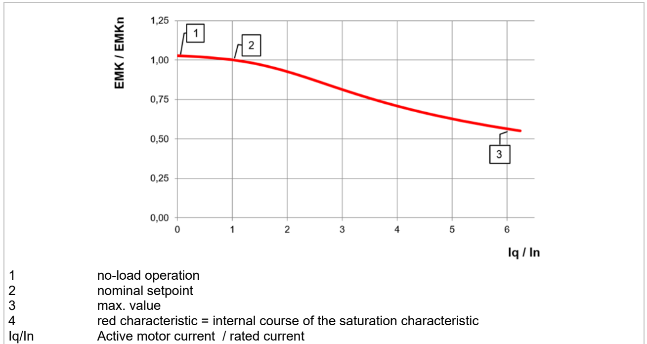
Figure 93: Torque constant depending on the active current
