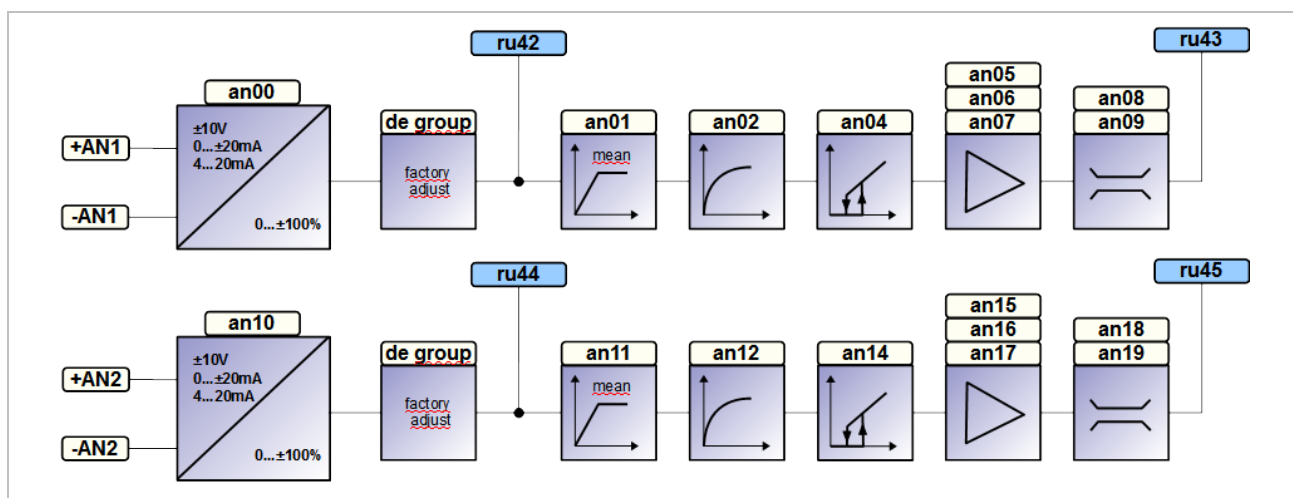
Figure 141: Analog inputs block diagram
