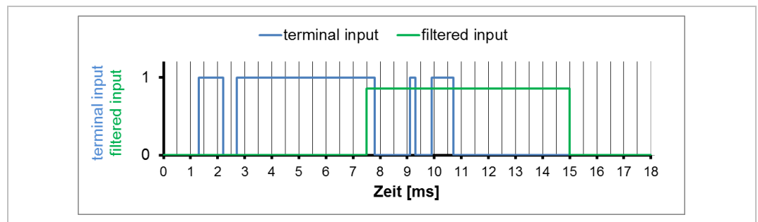
Figure 129: Filter of the digital inputs 2
