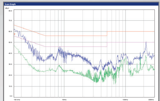
EMC characteristic
